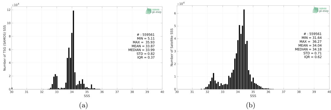
Figure 2: Histograms of SSS from TSG (SAMOS) (a) and SMAP SSS L3 v5 - Monthly (RSS) (b) considering all match-up pairs per bins of 0.1 over the Roaring Forties and Furious Fifties Pi-MEP region and for the full satellite product period.
