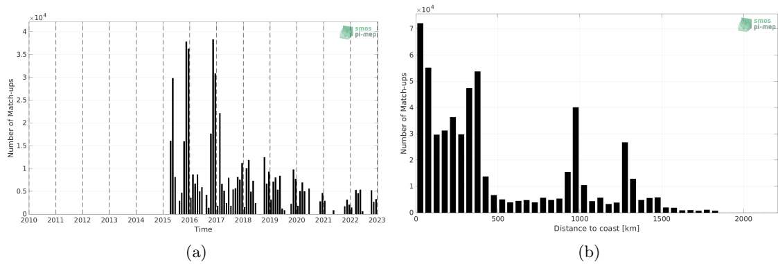
Figure 1: Number of match-ups between TSG (SAMOS) and SMAP SSS L3 v5 - Monthly (RSS) SSS as a function of time (a) and as function of the distance to coast (b) over the Roaring Forties and Furious Fifties Pi-MEP region and for the full satellite product period.
