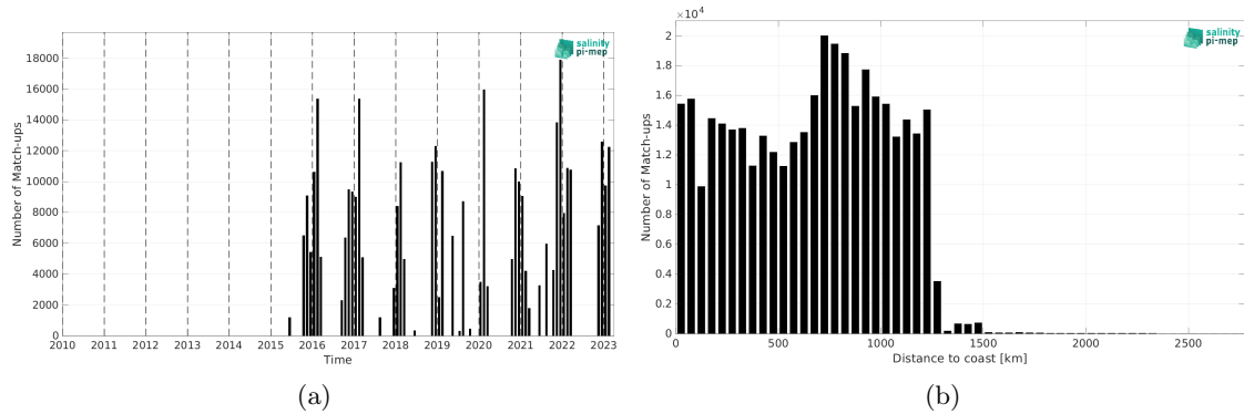
Figure 1: Number of match-ups between TSG (LEGOS-DM) and SMAP SSS L3 v5 - Monthly (RSS) SSS as a function of time (a) and as function of the distance to coast (b) over the Roaring Forties and Furious Fifties Pi-MEP region and for the full satellite product period.
