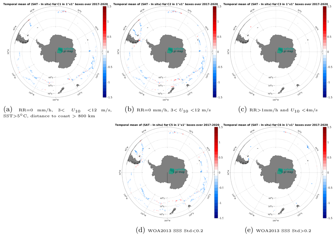
Figure 12: Temporal mean gridded over spatial boxes of size 1^\circ \times 1^\circ of \Delta\text{SSS} (SMAP SSS L3 v5 - Monthly (RSS) - TSG (GOSUD-Sailing-ship)) for 5 different subdatasets corresponding to: RR=0 mm/h, 3 < U_{10} < 12 m/s, SST > 5^\circ\text{C} , distance to coast > 800 km (a), RR=0 mm/h, 3 < U_{10} < 12 m/s (b), RR > 1 mm/h and U_{10} < 4 m/s (c), WOA2013 SSS Std < 0.2 (d), WOA2013 SSS Std > 0.2 (e).
