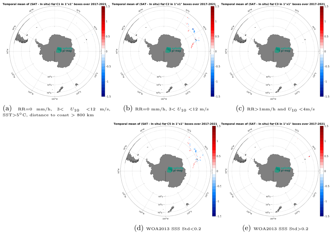
Figure 12: Temporal mean gridded over spatial boxes of size 1^\circ \times 1^\circ of \Delta\text{SSS} (SMAP SSS L3 v5 - Monthly (RSS) - TSG (GOSUD-Research-vessel)) for 5 different subdatasets corresponding to: RR=0 mm/h, 3 < U_{10} < 12 m/s, SST > 5^\circ\text{C} , distance to coast > 800 km (a), RR=0 mm/h, 3 < U_{10} < 12 m/s (b), RR > 1 mm/h and U_{10} < 4 m/s (c), WOA2013 SSS Std < 0.2 (d), WOA2013 SSS Std > 0.2 (e).
