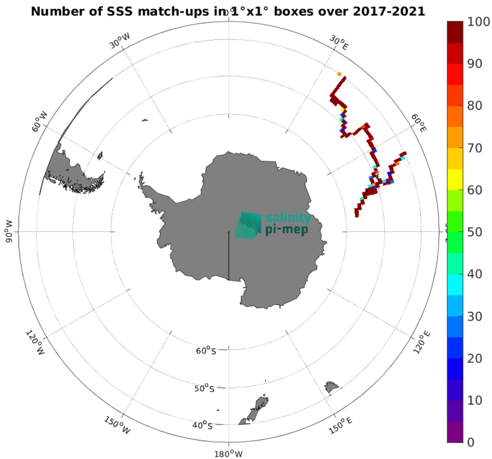
Figure 4: Number of SSS match-ups between TSG (GOSUD-Research-vessel) SSS and the SMAP SSS L3 v5 - Monthly (RSS) SSS product for the Roaring Forties and Furious Fifties Pi-MEP region over 1^{\circ} \times 1^{\circ} boxes and for the full satellite product period.
