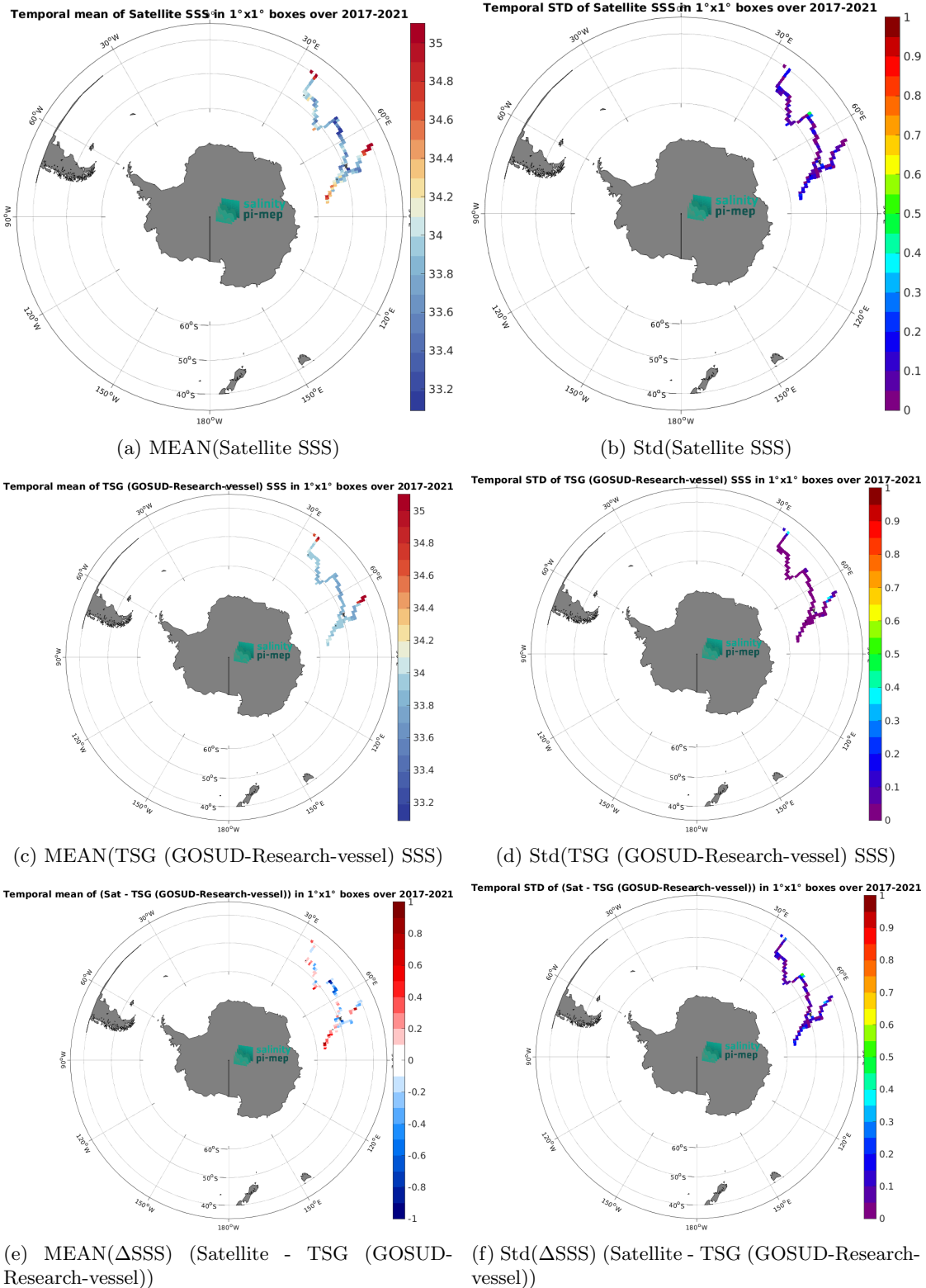
Figure 6: Temporal mean (left) and Std (right) of SSS from SMAP SSS L3 v5 - Monthly (RSS) (top), TSG (GOSUD-Research-vessel) (middle), and of \Delta SSS (Satellite - TSG (GOSUD-Research-vessel)). Only match-up pairs are used to generate these maps.
