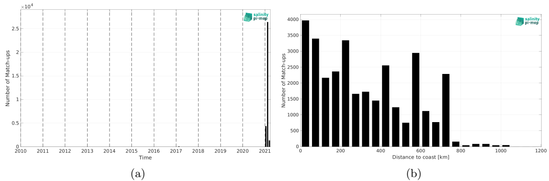
Figure 1: Number of match-ups between TSG (GOSUD-Research-vessel) and SMAP SSS L3 v5 - Monthly (RSS) SSS as a function of time (a) and as function of the distance to coast (b) over the Roaring Forties and Furious Fifties Pi-MEP region and for the full satellite product period.
