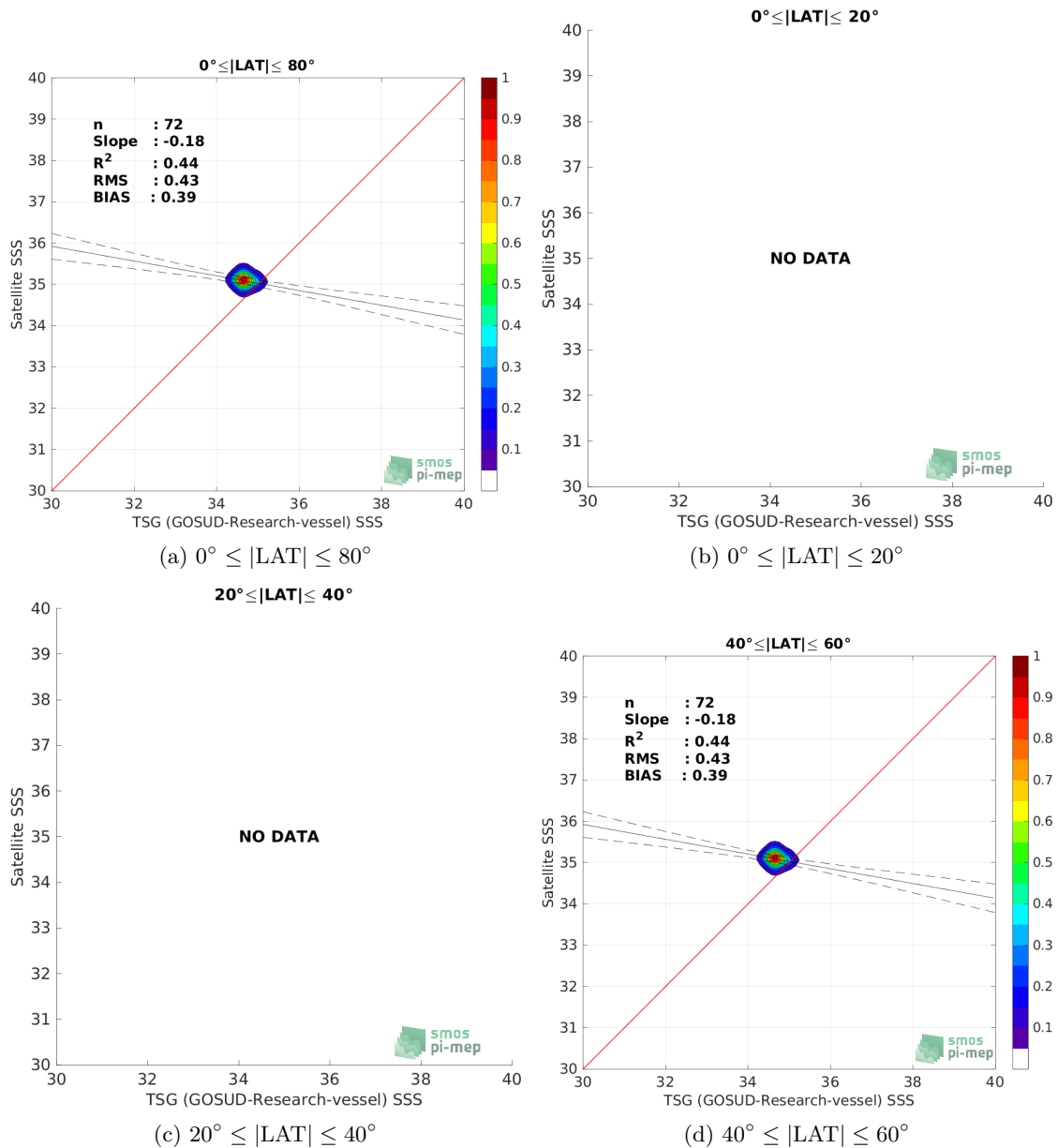
Figure 9: Contour maps of the concentration of SMAP SSS L3 v5 - Monthly (RSS) SSS (y-axis) versus TSG (GOSUD-Research-vessel) SSS (x-axis) at match-up pairs for different latitude bands. For each plot, the red line shows x=y . The black thin and dashed lines indicate a linear fit through the data cloud and the \pm 95\% confidence levels, respectively. The number match-up pairs n , the slope and R^2 coefficient of the linear fit, the root mean square (RMS) and the mean bias between satellite and in situ data are indicated for each latitude band in each plots.
