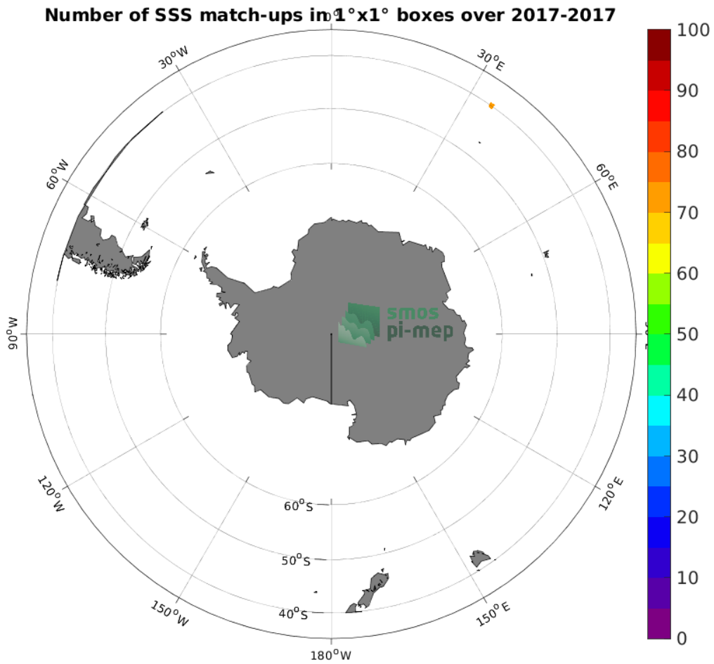
Figure 4: Number of SSS match-ups between TSG (GOSUD-Research-vessel) SSS and the SMAP SSS L3 v5 - Monthly (RSS) SSS product for the Roaring Forties and Furious Fifties Pi-MEP region over 1^\circ \times 1^\circ boxes and for the full satellite product period.
