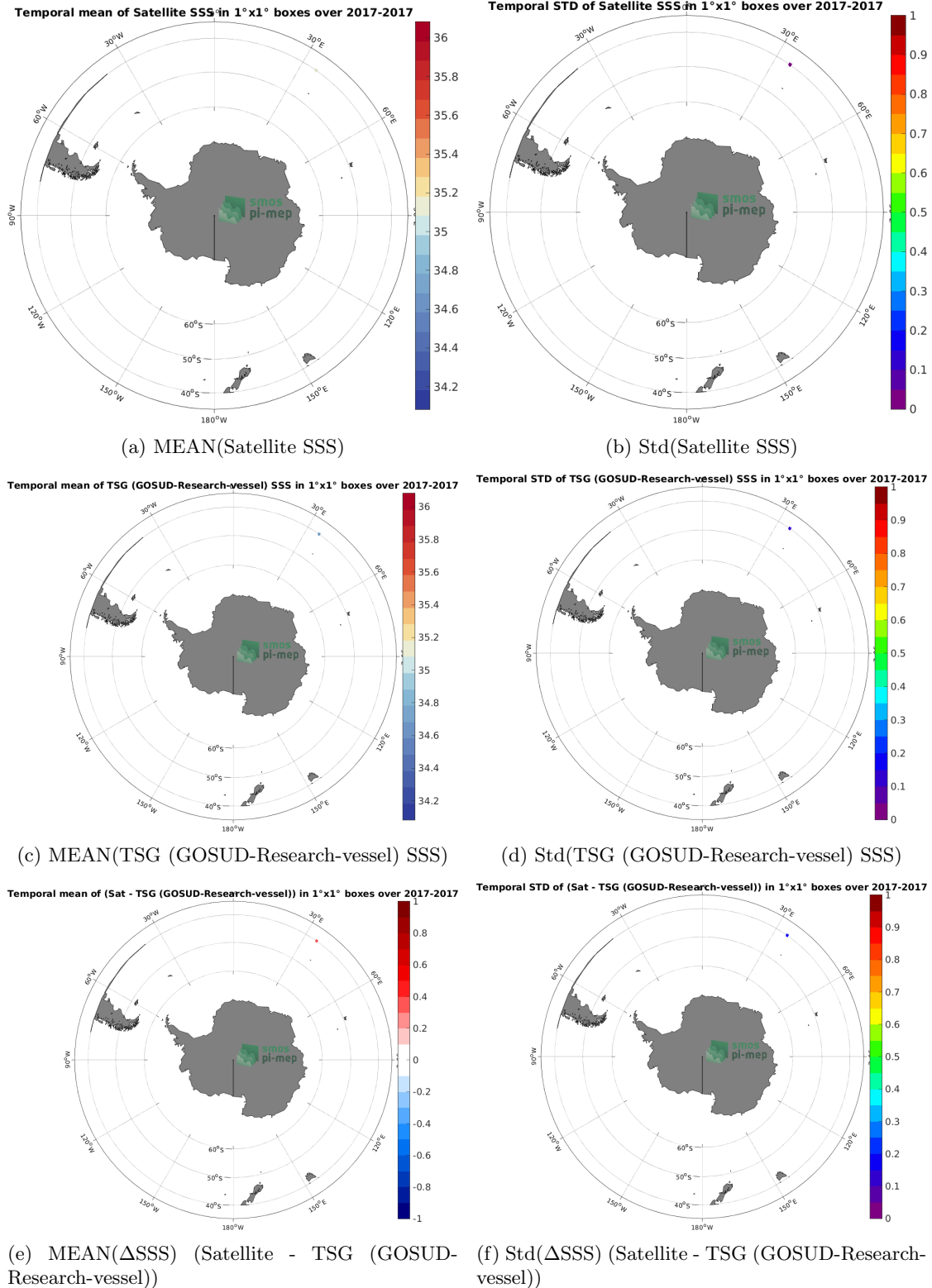
Figure 6: Temporal mean (left) and Std (right) of SSS from SMAP SSS L3 v5 - Monthly (RSS) (top), TSG (GOSUD-Research-vessel) (middle), and of \Delta SSS (Satellite - TSG (GOSUD-Research-vessel)). Only match-up pairs are used to generate these maps.
