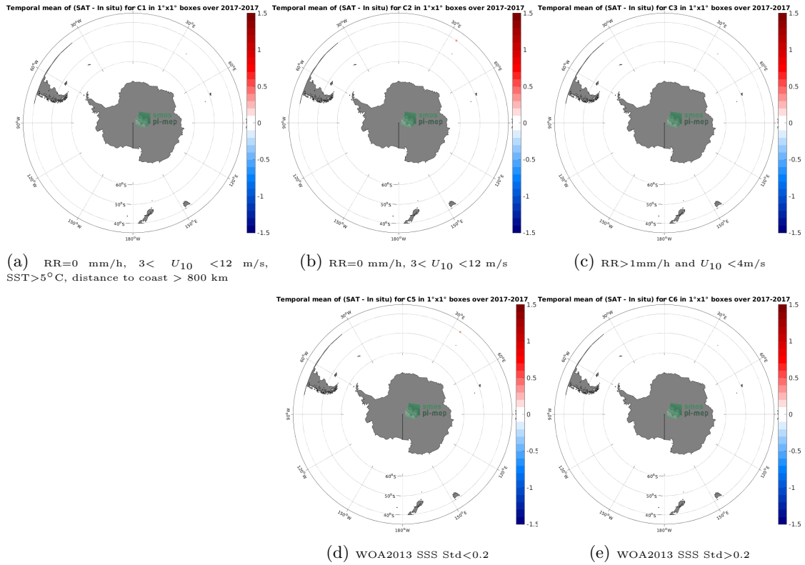
Figure 12: Temporal mean gridded over spatial boxes of size 1^\circ \times 1^\circ of \Delta SSS (SMAP SSS L3 v5 - Monthly (RSS) - TSG (GOSUD-Research-vessel)) for 5 different subdatasets corresponding to: RR=0 mm/h, 3 < U_{10} < 12 m/s, SST>5°C, distance to coast > 800 km (a), RR=0 mm/h, 3 < U_{10} < 12 m/s (b), RR>1mm/h and U_{10} < 4 m/s (c), WOA2013 SSS Std<0.2 (d), WOA2013 SSS Std>0.2 (e).
