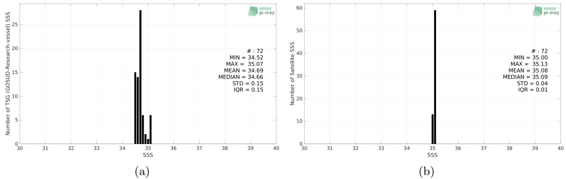
Figure 2: Histograms of SSS from TSG (GOSUD-Research-vessel) (a) and SMAP SSS L3 v5 - Monthly (RSS) (b) considering all match-up pairs per bins of 0.1 over the Roaring Forties and Furious Fifties Pi-MEP region and for the full satellite product period.
