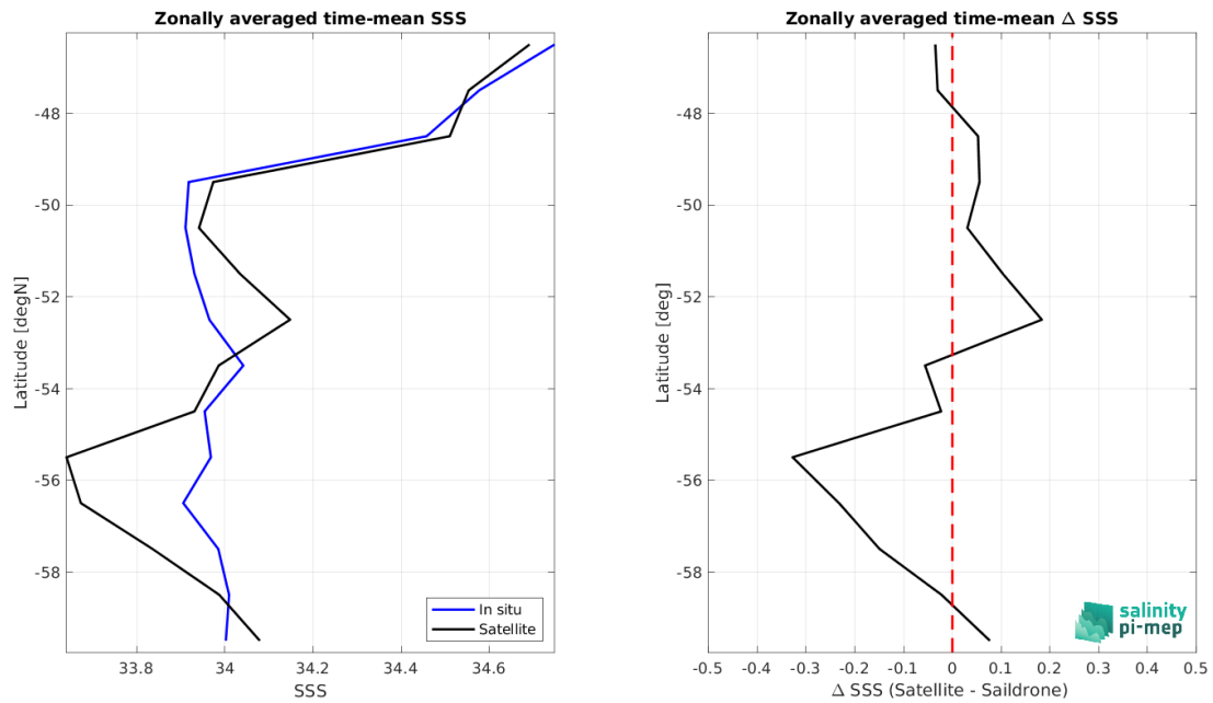
Figure 8: Left panel: Zonal mean SSS from SMAP SSS L3 v5 - Monthly (RSS) satellite product (black) and from Sairdrone (blue). Right panel: Zonal mean of \Delta SSS (Satellite - Sairdrone) for all the collected Pi-MEP match-up pairs estimated over the full satellite product period.
