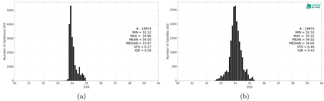
Figure 2: Histograms of SSS from Saildrone (a) and SMAP SSS L3 v5 - Monthly (RSS) (b) considering all match-up pairs per bins of 0.1 over the Roaring Forties and Furious Fifties Pi-MEP region and for the full satellite product period.
