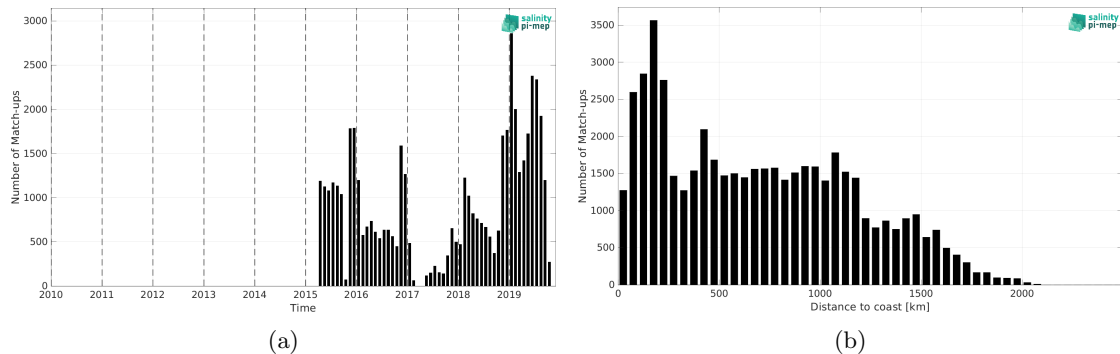
Figure 1: Number of match-ups between Marine mammals and SMAP SSS L3 v5 - Monthly (RSS) SSS as a function of time (a) and as function of the distance to coast (b) over the Roaring Forties and Furious Fifties Pi-MEP region and for the full satellite product period.
