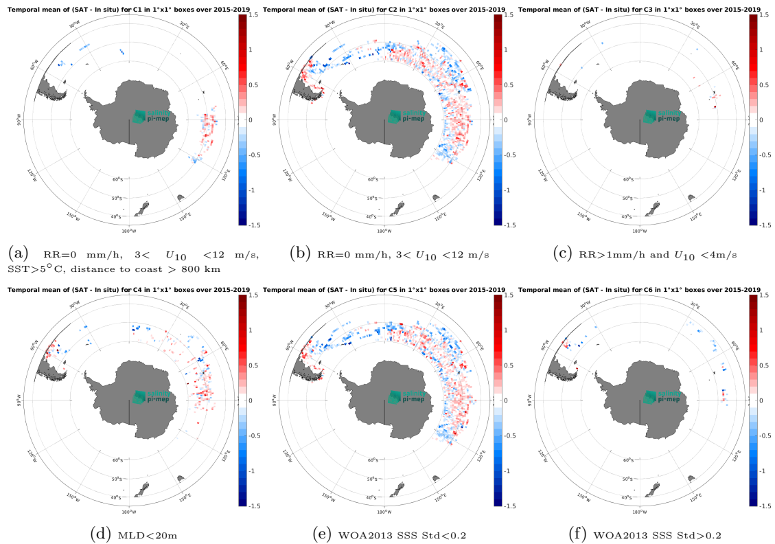
Figure 12: Temporal mean gridded over spatial boxes of size 1^{\circ}\times 1^{\circ} of \Delta\text{SSS} (SMAP SSS L3 v5 - Monthly (RSS) - Marine mammals) for 6 different subdatasets corresponding to:RR=0 mm/h, 3 < U_{10} < 12 m/s, SST >5^{\circ}\text{C} , distance to coast > 800 km (a), RR=0 mm/h, 3 < U_{10} < 12 m/s (b), RR >1 mm/h and U_{10} < 4 m/s (c),MLD <20 m (d),WOA2013 SSS Std <0.2 (e),WOA2013 SSS Std >0.2 (f).
