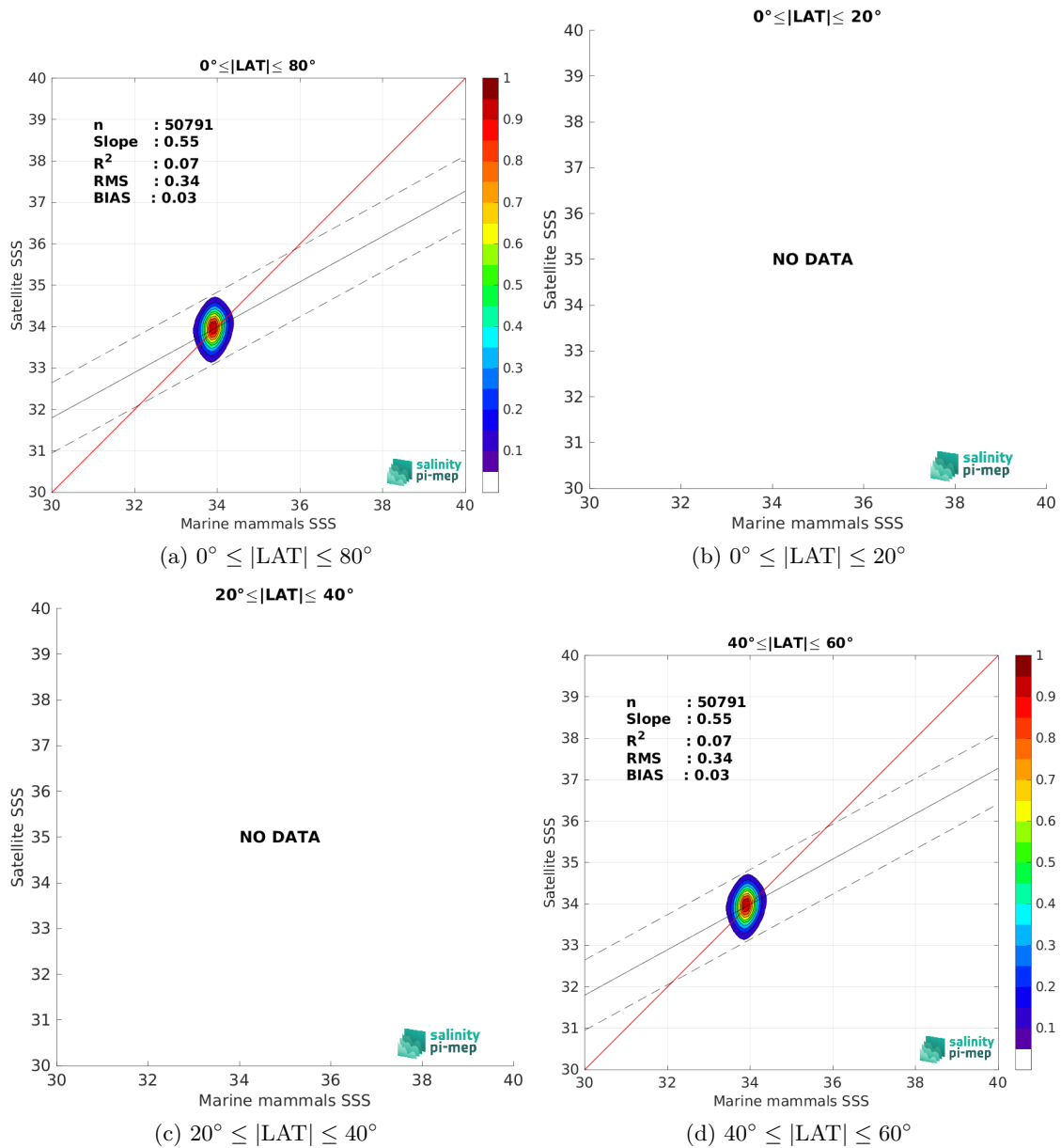
Figure 9: Contour maps of the concentration of SMAP SSS L3 v5 - Monthly (RSS) SSS (y-axis) versus Marine mammals SSS (x-axis) at match-up pairs for different latitude bands. For each plot, the red line shows x=y . The black thin and dashed lines indicate a linear fit through the data cloud and the \pm 95\% confidence levels, respectively. The number match-up pairs n , the slope and R^2 coefficient of the linear fit, the root mean square (RMS) and the mean bias between satellite and in situ data are indicated for each latitude band in each plots.
