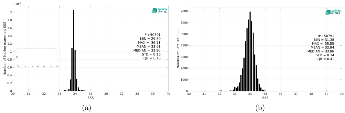
Figure 2: Histograms of SSS from Marine mammals (a) and SMAP SSS L3 v5 - Monthly (RSS) (b) considering all match-up pairs per bins of 0.1 over the Roaring Forties and Furious Fifties Pi-MEP region and for the full satellite product period.
