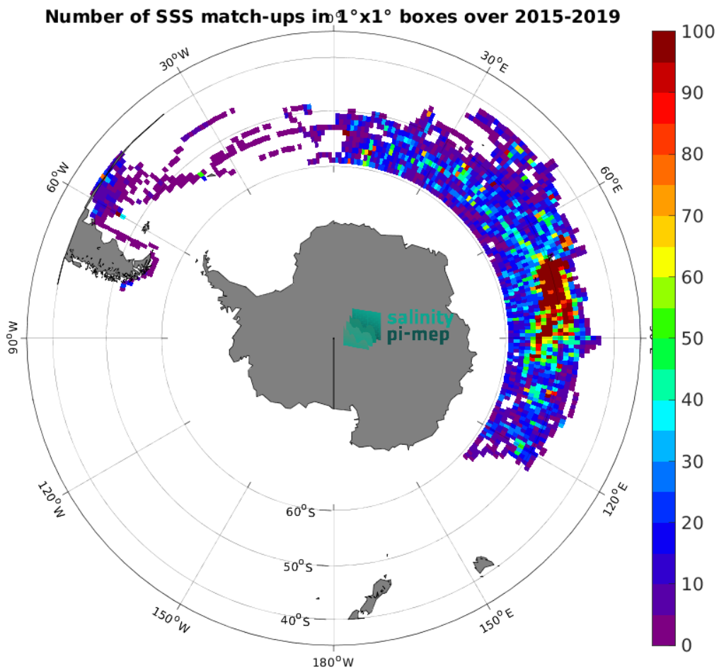
Figure 4: Number of SSS match-ups between Marine mammals SSS and the SMAP SSS L3 v5 - Monthly (RSS) SSS product for the Roaring Forties and Furious Fifties Pi-MEP region over 1^\circ \times 1^\circ boxes and for the full satellite product period.
