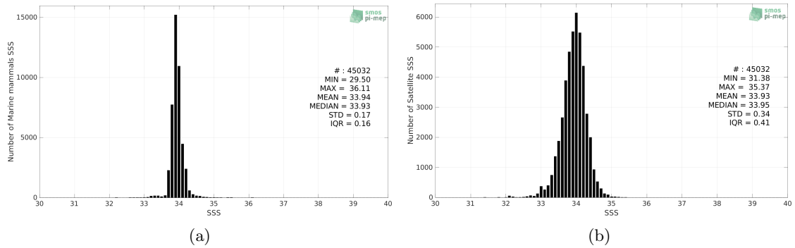
Figure 2: Histograms of SSS from Marine mammals (a) and SMAP SSS L3 v5 - Monthly (RSS) (b) considering all match-up pairs per bins of 0.1 over the Roaring Forties and Furious Fifties Pi-MEP region and for the full satellite product period.
