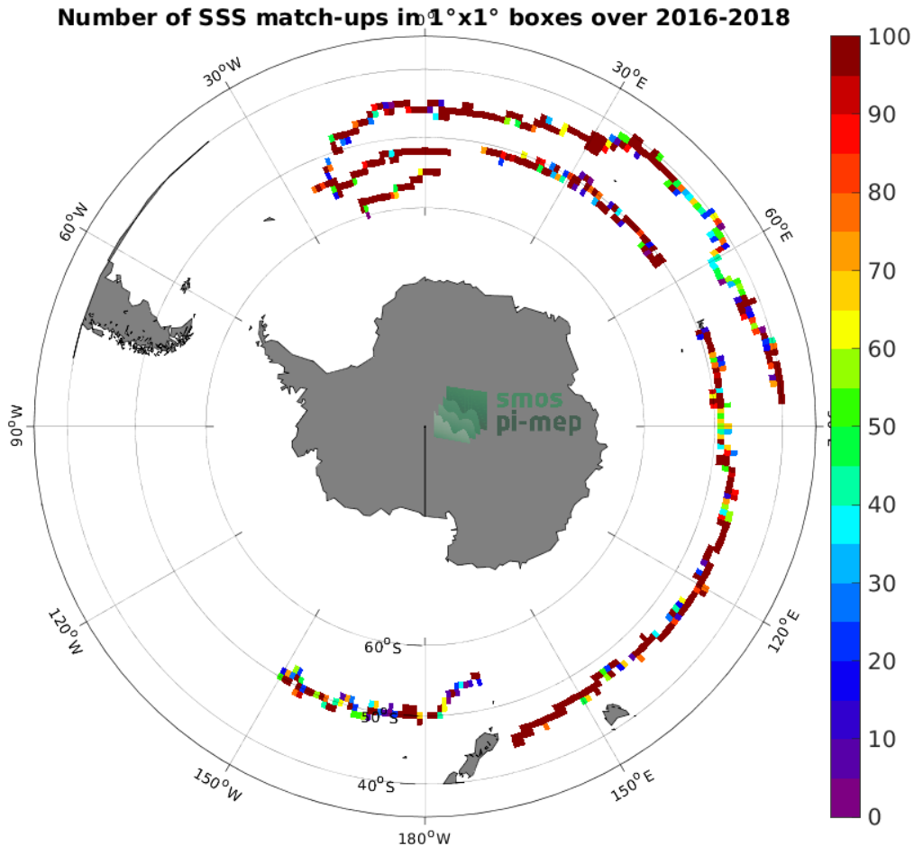
Figure 3: Number of SSS match-ups between Surface drifters SSS and the SMAP SSS L3 v5 - Monthly (RSS) SSS product for the Roaring Forties and Furious Fifties Pi-MEP region over 1^\circ \times 1^\circ boxes and for the full satellite product period.
