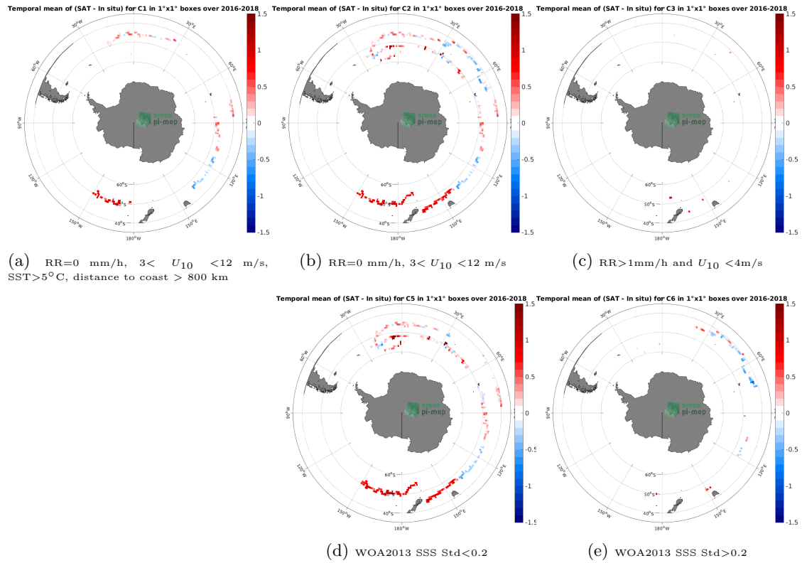
Figure 11: Temporal mean gridded over spatial boxes of size 1^{\circ}\times 1^{\circ} of \Delta\text{SSS} (SMAP SSS L3 v5 - Monthly (RSS) - Surface drifters) for 5 different subdatasets corresponding to: \text{RR}=0 mm/h, 3 < U_{10} < 12 m/s, \text{SST}>5^{\circ}\text{C} , distance to coast > 800 km (a), \text{RR}=0 mm/h, 3 < U_{10} < 12 m/s (b), \text{RR}>1 mm/h and U_{10} < 4 m/s (c), WOA2013 SSS Std < 0.2 (d), WOA2013 SSS Std > 0.2 (e).
