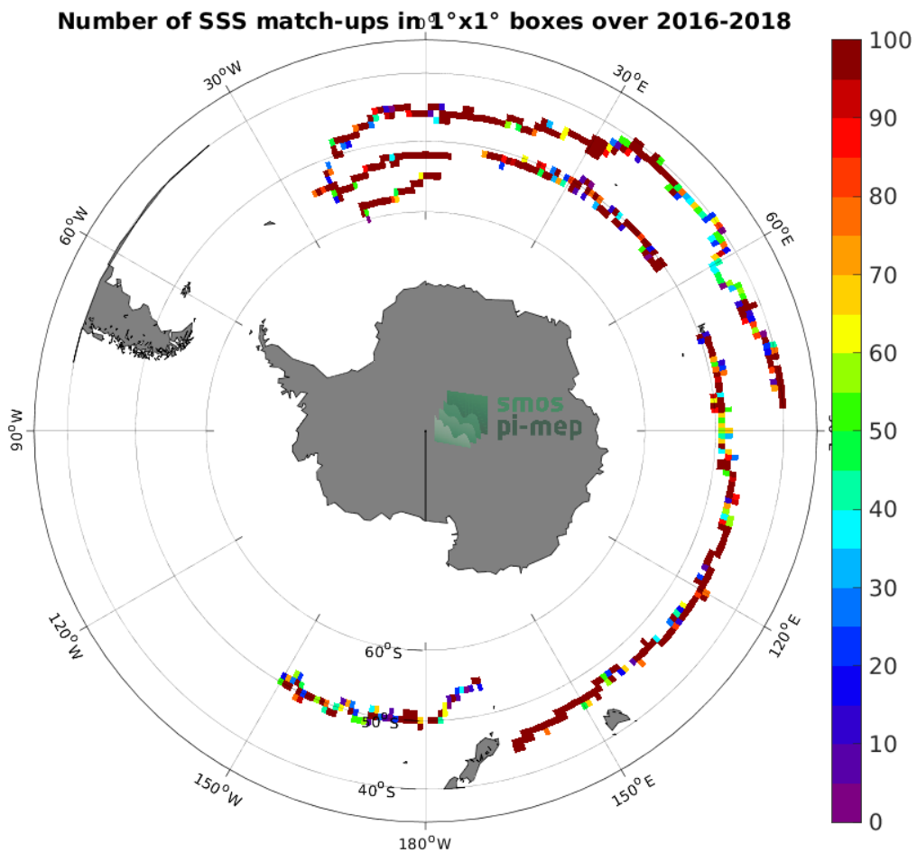
Figure 3: Number of SSS match-ups between Surface drifters SSS and the SMAP SSS L3 v5 - Monthly (RSS) SSS product for the Roaring Forties and Furious Fifties Pi-MEP region over 1^\circ \times 1^\circ boxes and for the full satellite product period.
