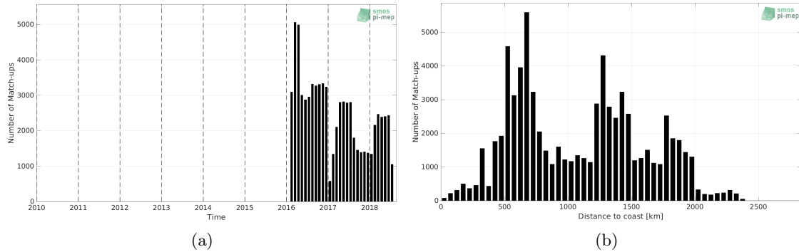
Figure 1: Number of match-ups between Surface drifters and SMAP SSS L3 v5 - Monthly (RSS) SSS as a function of time (a) and as function of the distance to coast (b) over the Roaring Forties and Furious Fifties Pi-MEP region and for the full satellite product period.
