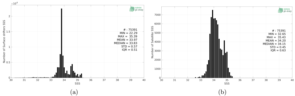
Figure 2: Histograms of SSS from Surface drifters (a) and SMAP SSS L3 v5 - Monthly (RSS) (b) considering all match-up pairs per bins of 0.1 over the Roaring Forties and Furious Fifties Pi-MEP region and for the full satellite product period.
