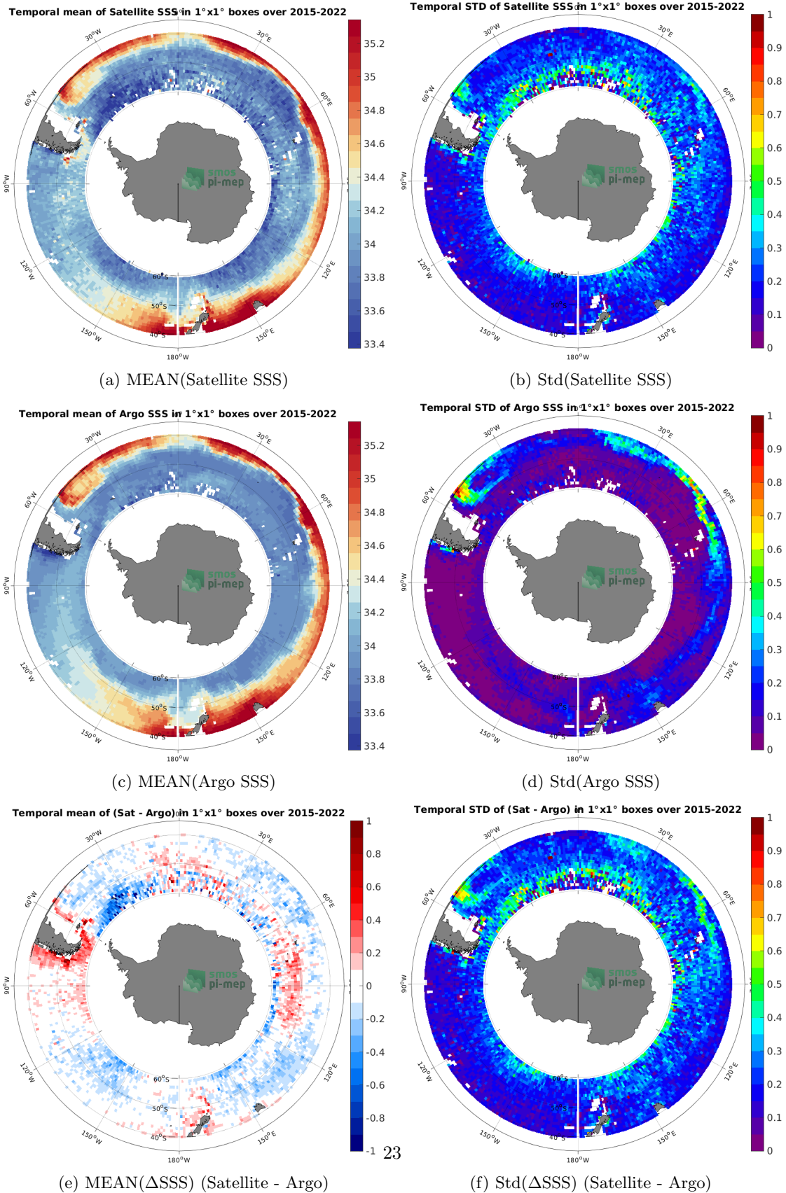
Figure 6: Temporal mean (left) and Std (right) of SSS from SMAP SSS L3 v5 - Monthly (RSS) (top), Argo (middle), and of \Delta SSS (Satellite - Argo). Only match-up pairs are used to generate these maps.
