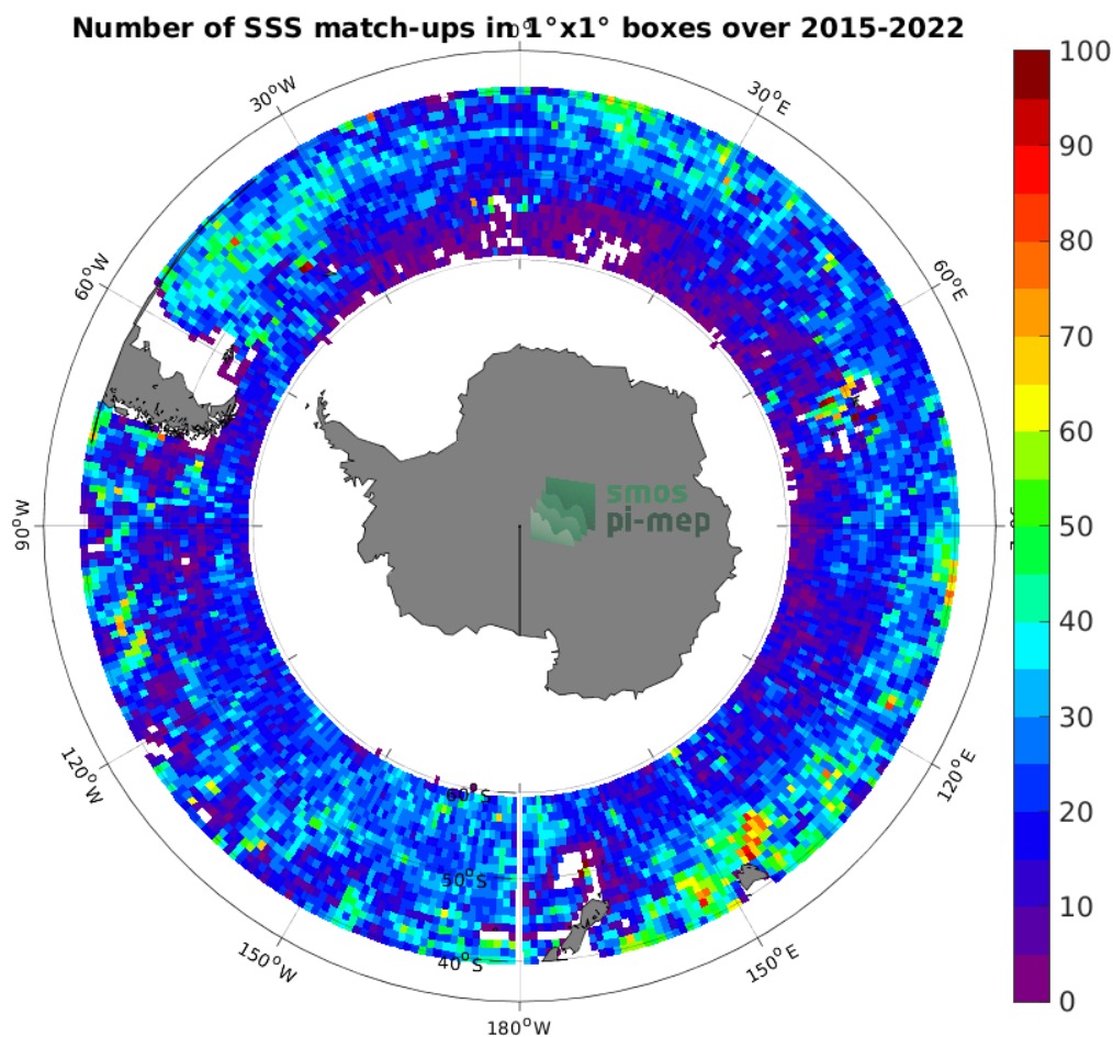
Figure 4: Number of SSS match-ups between Argo SSS and the SMAP SSS L3 v5 - Monthly (RSS) SSS product for the Roaring Forties and Furious Fifties Pi-MEP region over 1^\circ \times 1^\circ boxes and for the full satellite product period.
