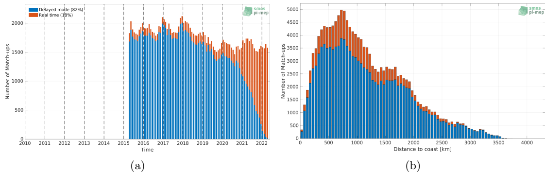
Figure 1: Number of match-ups between Argo and SMAP SSS L3 v5 - Monthly (RSS) SSS as a function of time (a) and as function of the distance to coast (b) over the Roaring Forties and Furious Fifties Pi-MEP region and for the full satellite product period.
