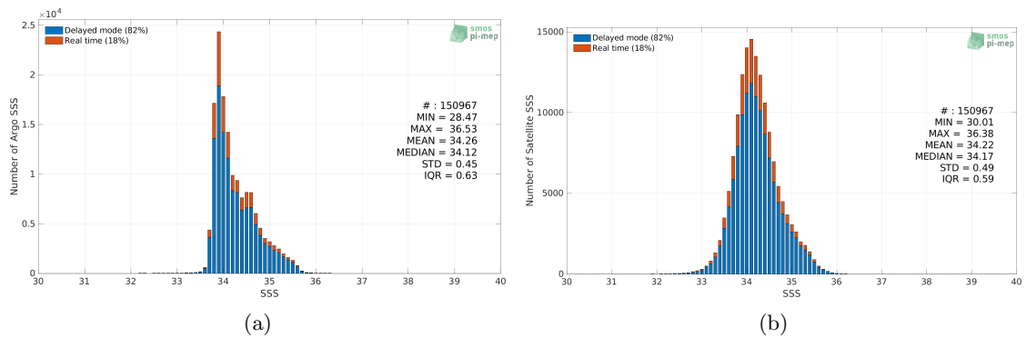
Figure 2: Histograms of SSS from Argo (a) and SMAP SSS L3 v5 - Monthly (RSS) (b) considering all match-up pairs per bins of 0.1 over the Roaring Forties and Furious Fifties Pi-MEP region and for the full satellite product period.
