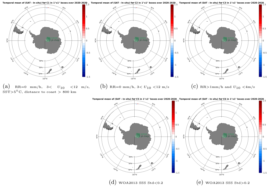
Figure 12: Temporal mean gridded over spatial boxes of size 1^{\circ}\times 1^{\circ} of \Delta\text{SSS} (SMAP SSS L3 v4 - 8-Day running (RSS) - TSG (SAMOS)) for 5 different subdatasets corresponding to:RR=0 mm/h, 3 < U_{10} < 12 m/s, SST >5^{\circ}\text{C} , distance to coast > 800 km (a), RR=0 mm/h, 3 < U_{10} < 12 m/s (b), RR >1 mm/h and U_{10} < 4 m/s (c), WOA2013 SSS Std <0.2 (d), WOA2013 SSS Std >0.2 (e).
