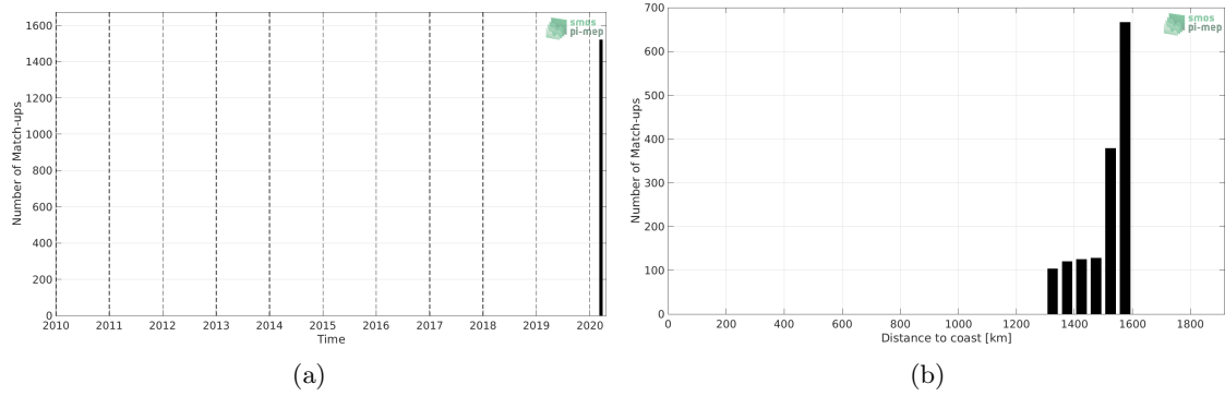
Figure 1: Number of match-ups between TSG (SAMOS) and SMAP SSS L3 v4 - 8-Day running (RSS) SSS as a function of time (a) and as function of the distance to coast (b) over the Roaring Forties and Furious Fifties Pi-MEP region and for the full satellite product period.
