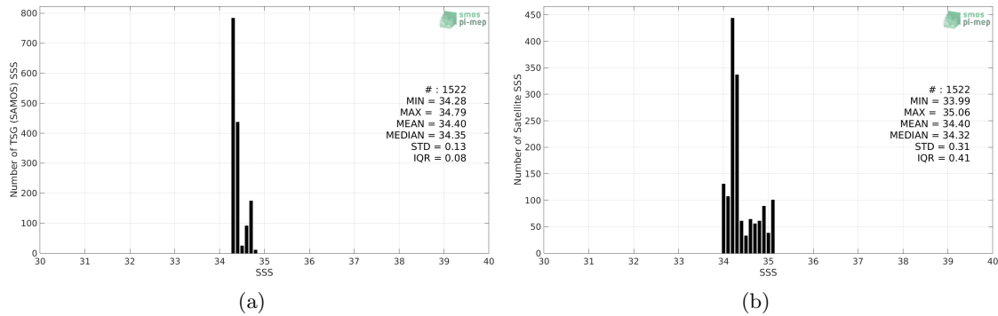
Figure 2: Histograms of SSS from TSG (SAMOS) (a) and SMAP SSS L3 v4 - 8-Day running (RSS) (b) considering all match-up pairs per bins of 0.1 over the Roaring Forties and Furious Fifties Pi-MEP region and for the full satellite product period.
