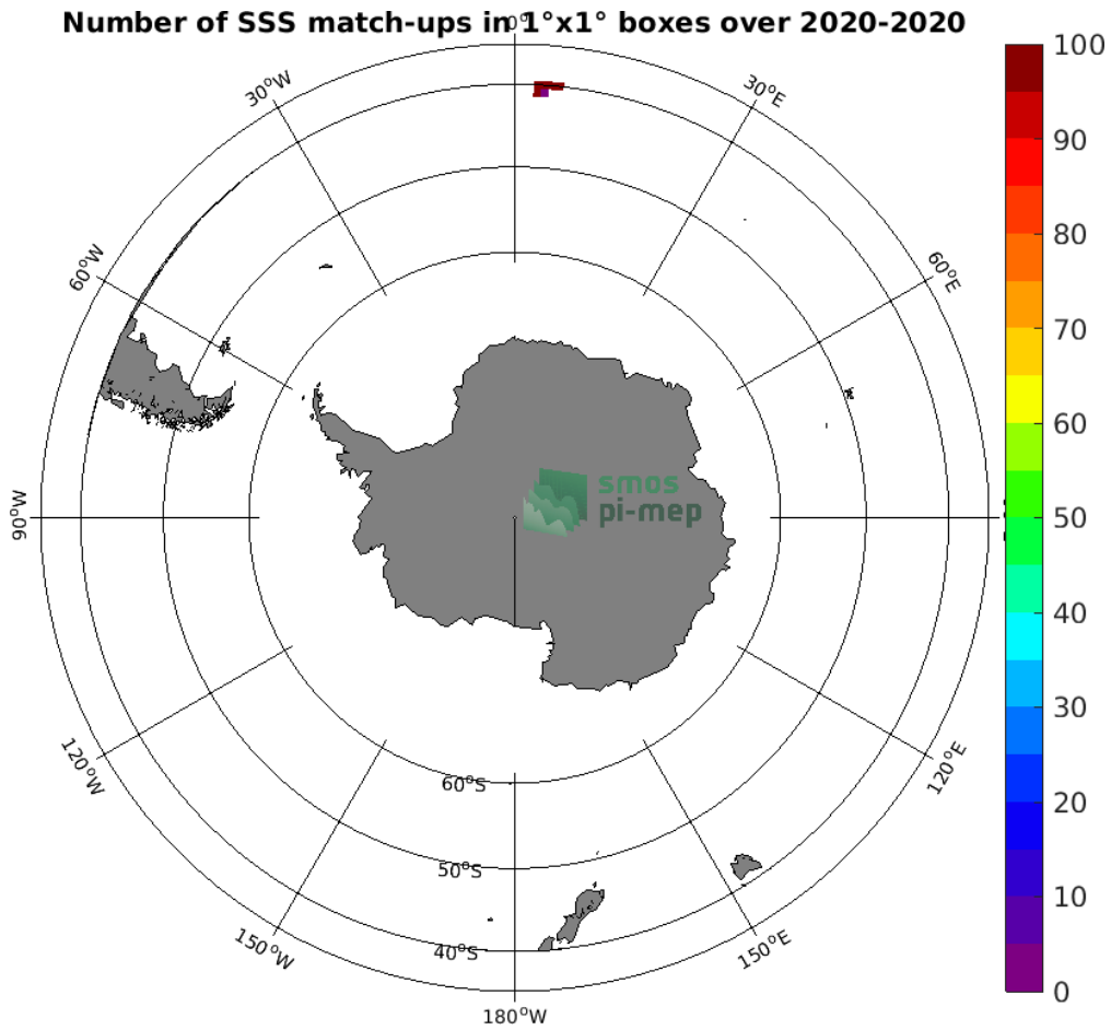
Figure 4: Number of SSS match-ups between TSG (SAMOS) SSS and the SMAP SSS L3 v4 - 8-Day running (RSS) SSS product for the Roaring Forties and Furious Fifties Pi-MEP region over 1°x1° boxes and for the full satellite product period.
