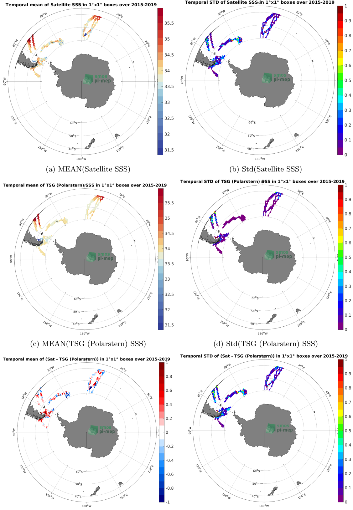
Figure 6: Temporal mean (left) and Std (right) of SSS from SMAP SSS L3 v4 - 8-Day running (RSS) (top), TSG (Polarstern) (middle), and of \Delta SSS (Satellite - TSG (Polarstern)). Only match-up pairs are used to generate these maps.
