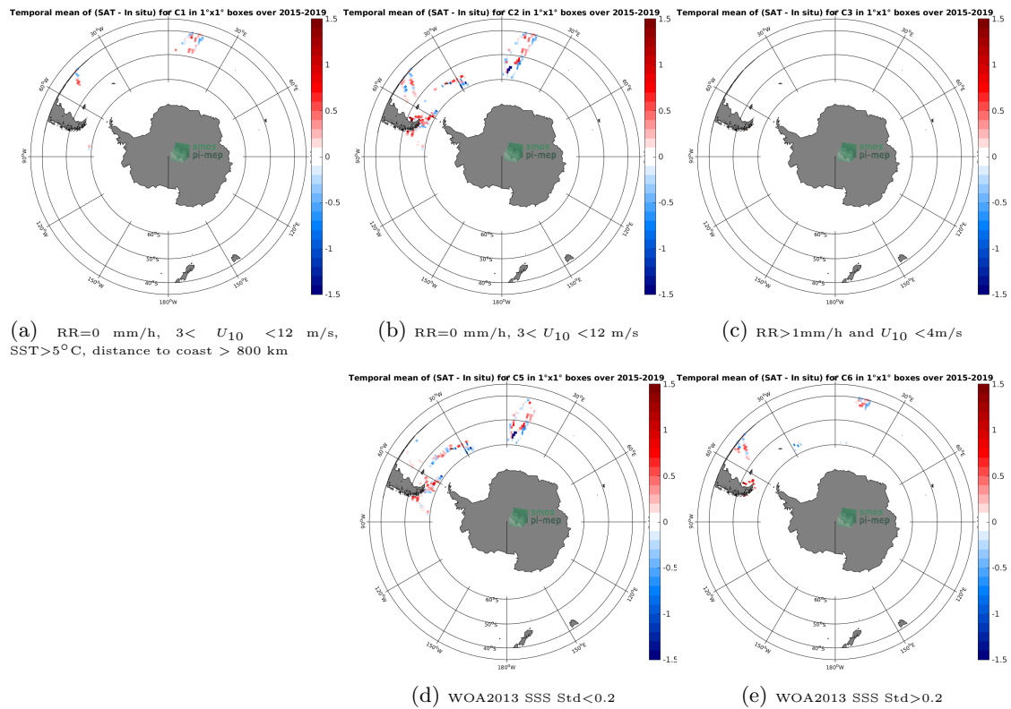
Figure 12: Temporal mean gridded over spatial boxes of size 1^{\circ}\times 1^{\circ} of \Delta\text{SSS} (SMAP-L3-RSS-V4-8DAY-RUNNING - TSG-POLARSTERN) for 5 different subdatasets corresponding to:RR=0 mm/h, 3 < U_{10} < 12 m/s, SST >5^{\circ}\text{C} , distance to coast > 800 km (a), RR=0 mm/h, 3 < U_{10} < 12 m/s (b), RR >1 mm/h and U_{10} < 4 m/s (c), WOA2013 SSS Std <0.2 (d), WOA2013 SSS Std >0.2 (e).
