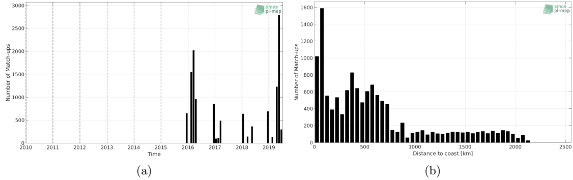
Figure 1: Number of match-ups between TSG-POLARSTERN and SMAP-L3-RSS-V4-8DAY-RUNNING SSS as a function of time (a) and as function of the distance to coast (b) over the Roaring Forties and Furious Fifties Pi-MEP region and for the full satellite product period.
