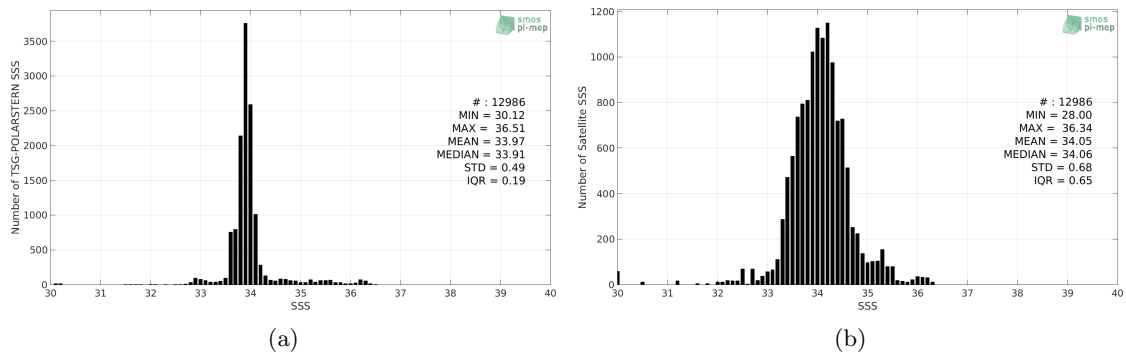
Figure 2: Histograms of SSS from TSG-POLARSTERN (a) and SMAP-L3-RSS-V4-8DAY-RUNNING (b) considering all match-up pairs per bins of 0.1 over the Roaring Forties and Furious Fifties Pi-MEP region and for the full satellite product period.
