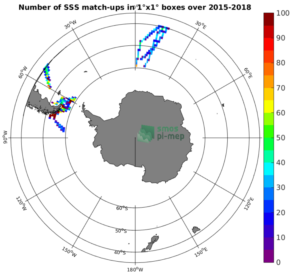
Figure 4: Number of SSS match-ups between TSG-POLARSTERN SSS and the SMAP-L3-RSS-V4-8DAY-RUNNING SSS product for the Roaring Forties and Furious Fifties Pi-MEP region over 1°x1° boxes and for the full satellite product period.
