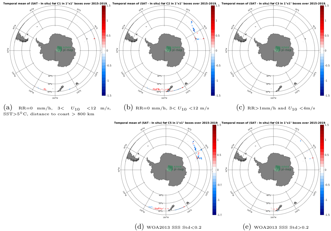
Figure 12: Temporal mean gridded over spatial boxes of size 1^{\circ}\times 1^{\circ} of \Delta\text{SSS} (SMAP-L3-RSS-V4-8DAY-RUNNING - TSG-LEGOS-DM) for 5 different subdatasets corresponding to:RR=0 mm/h, 3 < U_{10} < 12 m/s, SST >5^{\circ}\text{C} , distance to coast > 800 km (a), RR=0 mm/h, 3 < U_{10} < 12 m/s (b), RR >1 mm/h and U_{10} < 4 m/s (c), WOA2013 SSS Std <0.2 (d), WOA2013 SSS Std >0.2 (e).
