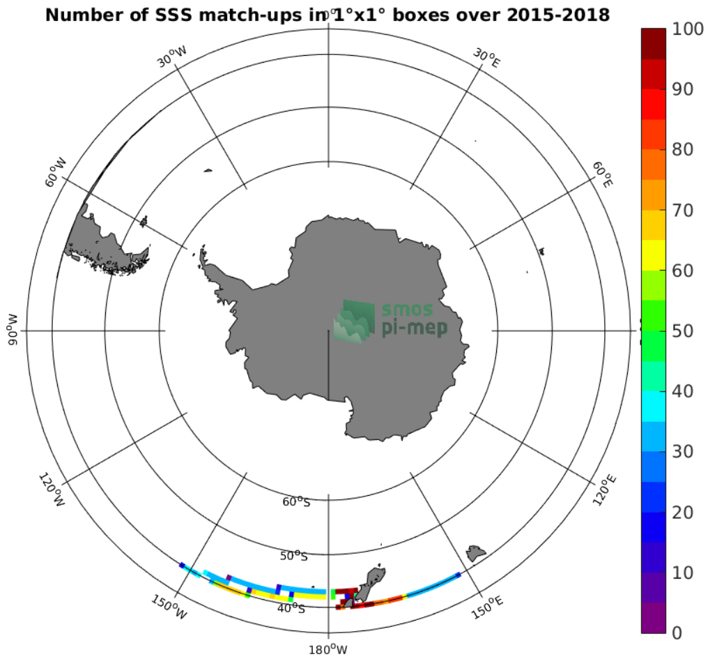
Figure 4: Number of SSS match-ups between TSG-LEGOS-DM SSS and the SMAP-L3-RSS-V4-8DAY-RUNNING SSS product for the Roaring Forties and Furious Fifties Pi-MEP region over 1°x1° boxes and for the full satellite product period.
