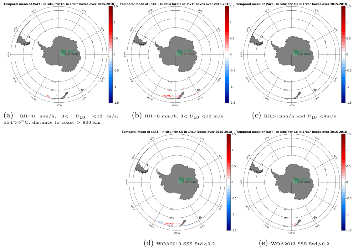
Figure 12: Temporal mean gridded over spatial boxes of size 1^\circ \times 1^\circ of \Delta SSS (SMAP-L3-RSS-V4-8DAY-RUNNING - TSG-LEGOS-DM) for 5 different subdatasets corresponding to:RR=0 mm/h, 3 < U_{10} < 12 m/s, SST>5°C, distance to coast > 800 km (a), RR=0 mm/h, 3 < U_{10} < 12 m/s (b), RR>1mm/h and U_{10} < 4 m/s (c), WOA2013 SSS Std<0.2 (d), WOA2013 SSS Std>0.2 (e).
