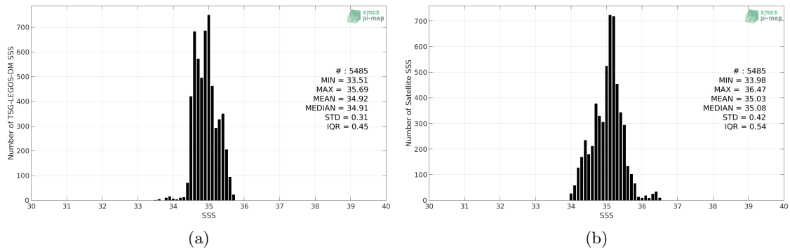
Figure 2: Histograms of SSS from TSG-LEGOS-DM (a) and SMAP-L3-RSS-V4-8DAY-RUNNING (b) considering all match-up pairs per bins of 0.1 over the Roaring Forties and Furious Fifties Pi-MEP region and for the full satellite product period.
