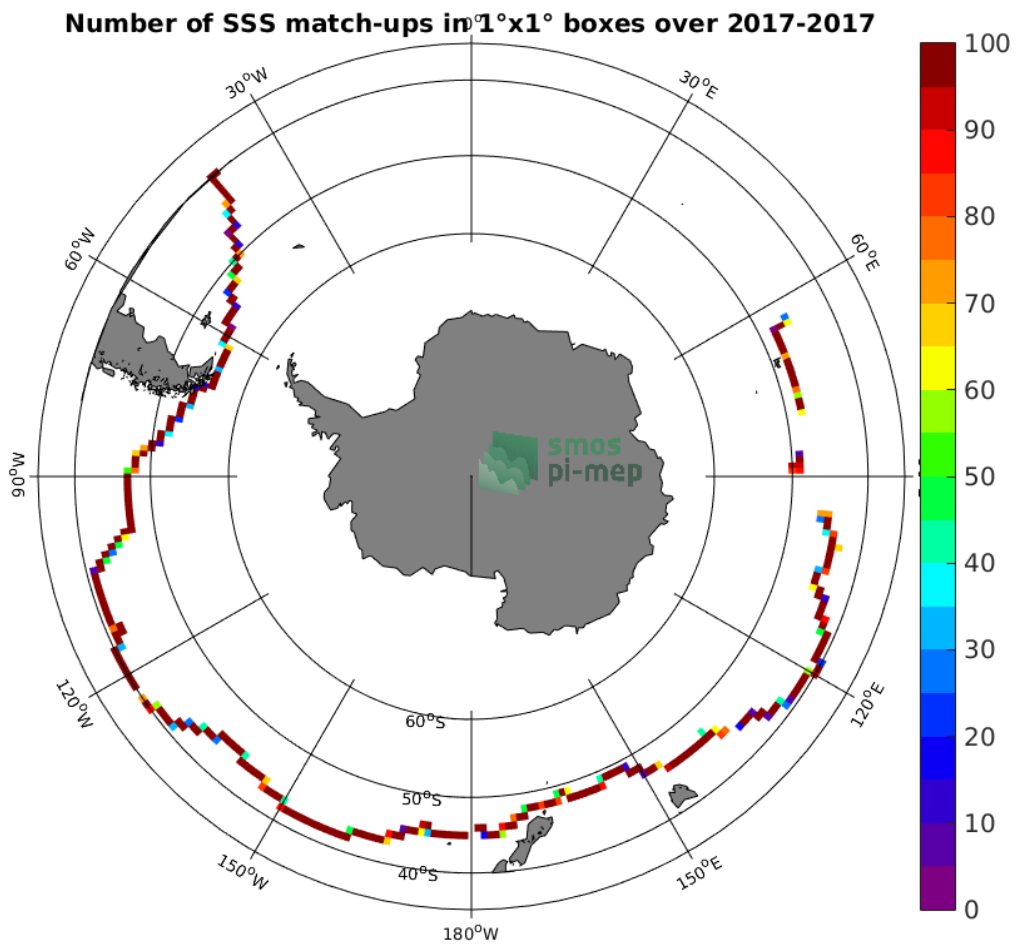
Figure 4: Number of SSS match-ups between TSG-GOSUD-Sailing-ship SSS and the SMAP-L3-RSS-V4-8DAY-RUNNING SSS product for the Roaring Forties and Furious Fifties Pi-MEP region over 1^\circ \times 1^\circ boxes and for the full satellite product period.
