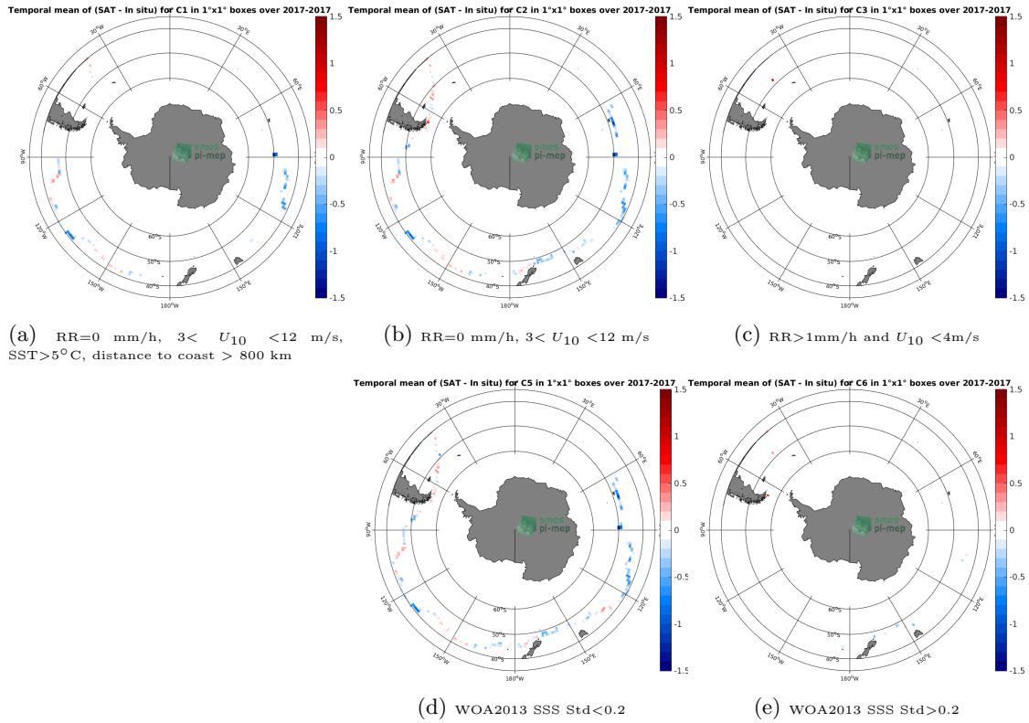
Figure 12: Temporal mean gridded over spatial boxes of size 1°x1° of \Delta SSS (SMAP-L3-RSS-V4-8DAY-RUNNING - TSG-GOSUD-Sailing-ship) for 5 different subdatasets corresponding to:RR=0 mm/h, 3 < U_{10} < 12 m/s, SST>5°C, distance to coast > 800 km (a), RR=0 mm/h, 3 < U_{10} < 12 m/s (b), RR>1mm/h and U_{10} < 4 m/s (c), WOA2013 SSS Std<0.2 (d), WOA2013 SSS Std>0.2 (e).
