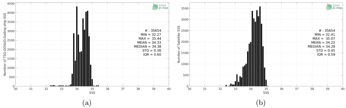
Figure 2: Histograms of SSS from TSG-GOSUD-Sailing-ship (a) and SMAP-L3-RSS-V4-8DAY-RUNNING (b) considering all match-up pairs per bins of 0.1 over the Roaring Forties and Furious Fifties Pi-MEP region and for the full satellite product period.
