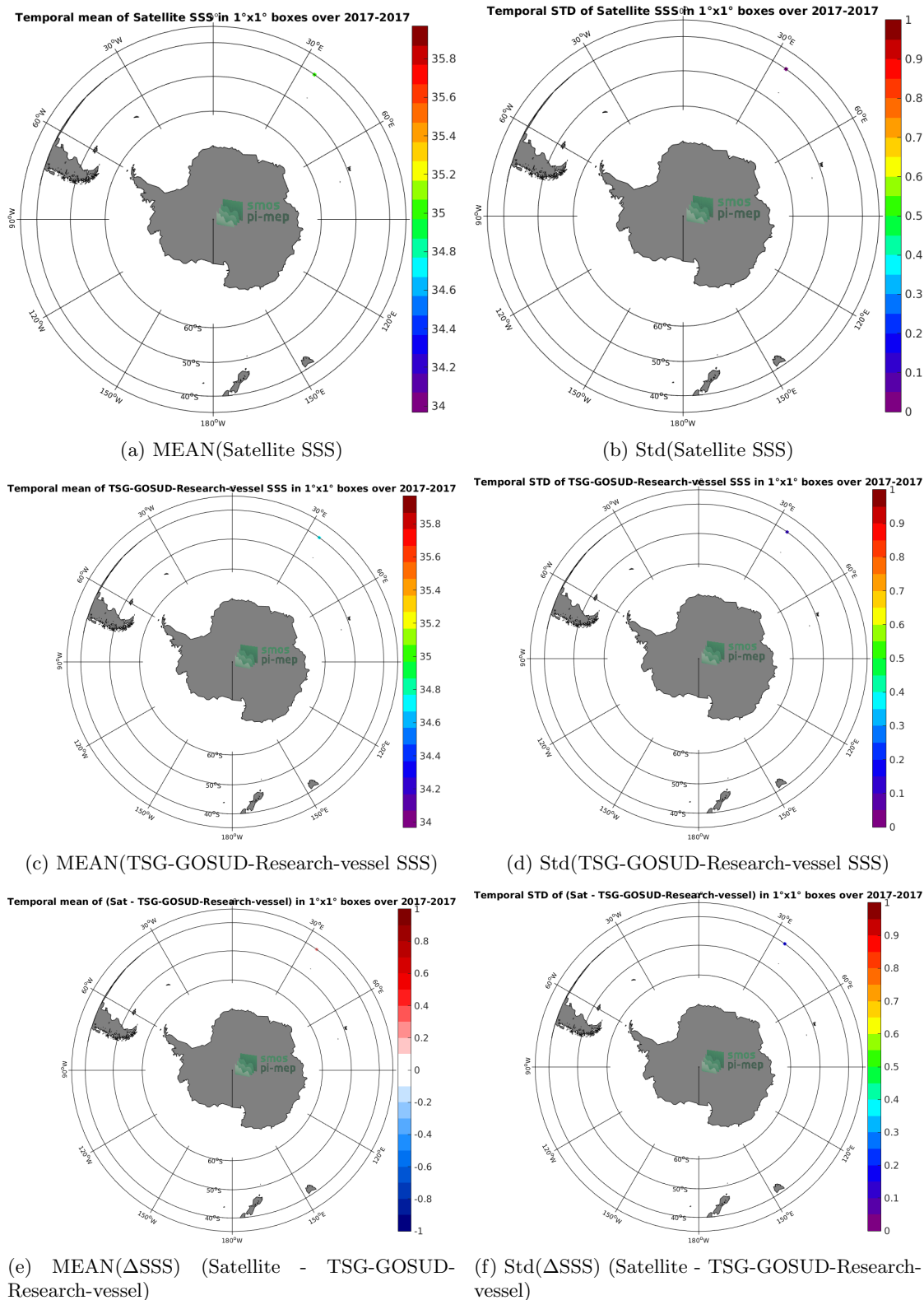
Figure 6: Temporal mean (left) and Std (right) of SSS from SMAP-L3-RSS-V4-8DAY-RUNNING (top), TSG-GOSUD-Research-vessel (middle), and of \Delta SSS (Satellite - TSG-GOSUD-Research-vessel). Only match-up pairs are used to generate these maps.
