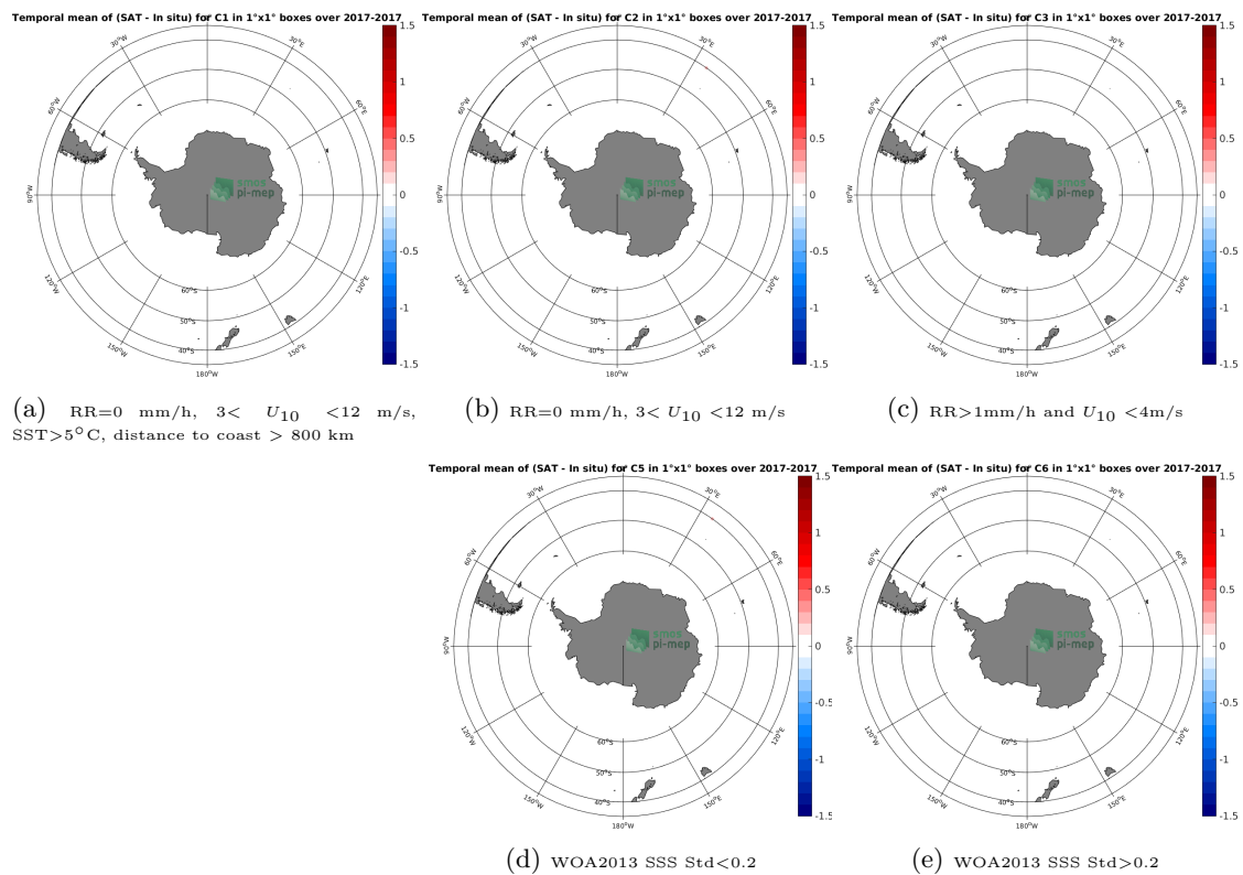
Figure 12: Temporal mean gridded over spatial boxes of size 1^\circ \times 1^\circ of \Delta SSS (SMAP-L3-RSS-V4-8DAY-RUNNING - TSG-GOSUD-Research-vessel) for 5 different subdatasets corresponding to:RR=0 mm/h, 3 < U_{10} < 12 m/s, SST>5°C, distance to coast > 800 km (a), RR=0 mm/h, 3 < U_{10} < 12 m/s (b), RR>1mm/h and U_{10} < 4 m/s (c), WOA2013 SSS Std<0.2 (d), WOA2013 SSS Std>0.2 (e).
