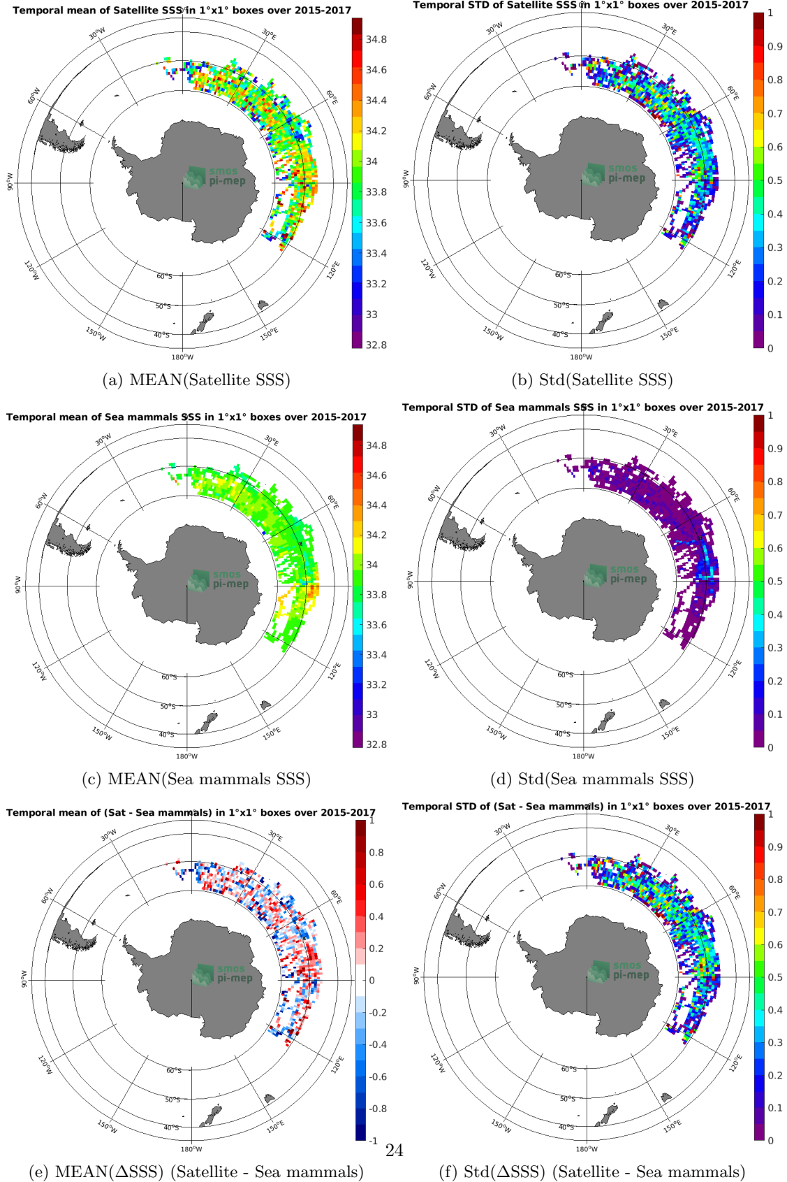
Figure 6: Temporal mean (left) and Std (right) of SSS from SMAP SSS L3 v4 - 8-Day running (RSS) (top), Sea mammals (middle), and of \Delta SSS (Satellite - Sea mammals). Only match-up pairs are used to generate these maps.
