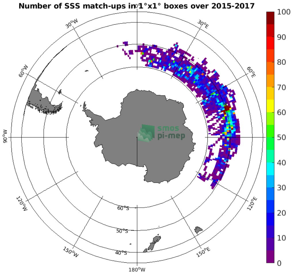
Figure 4: Number of SSS match-ups between Sea mammals SSS and the SMAP SSS L3 v4 - 8-Day running (RSS) SSS product for the Roaring Forties and Furious Fifties Pi-MEP region over 1^\circ \times 1^\circ boxes and for the full satellite product period.
