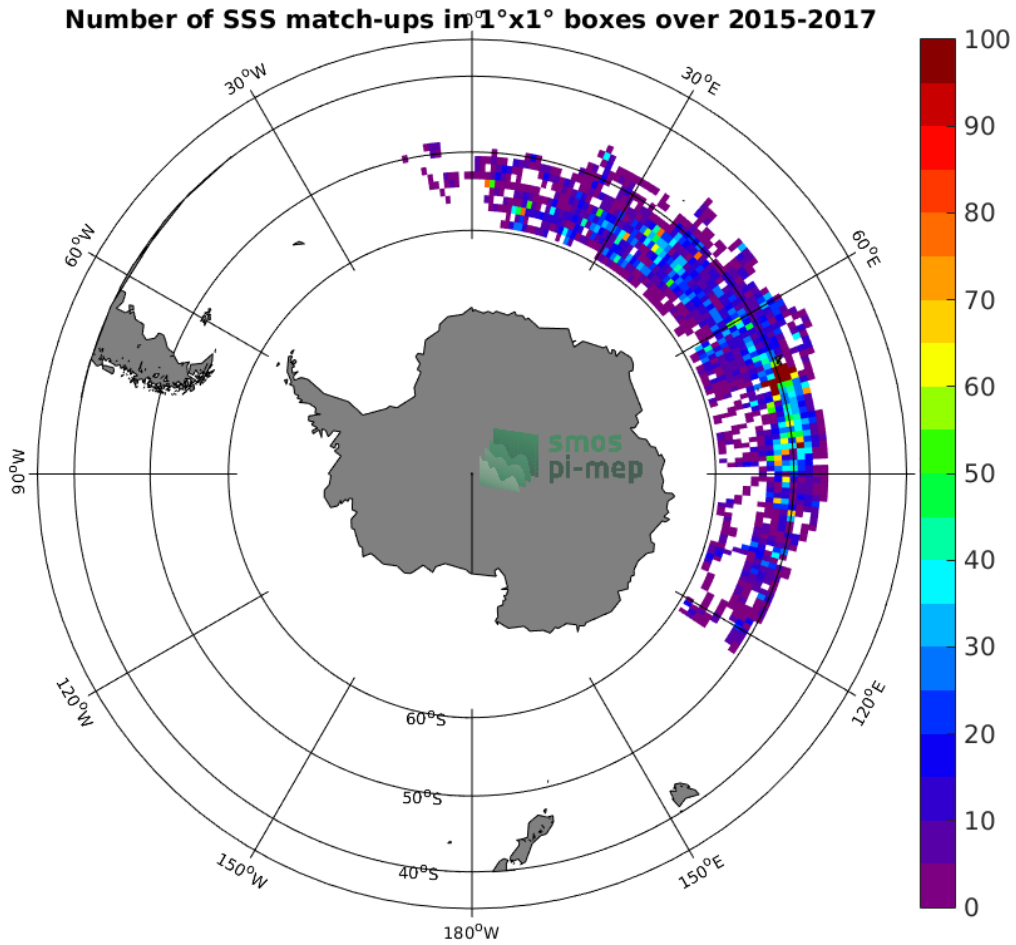
Figure 4: Number of SSS match-ups between Sea mammals SSS and the SMAP-L3-RSS-V4-8DAY-RUNNING SSS product for the Roaring Forties and Furious Fifties Pi-MEP region over 1°x1° boxes and for the full satellite product period.
