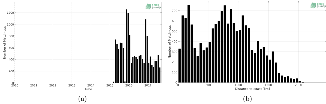
Figure 1: Number of match-ups between Sea mammals and SMAP-L3-RSS-V4-8DAY-RUNNING SSS as a function of time (a) and as function of the distance to coast (b) over the Roaring Forties and Furious Fifties Pi-MEP region and for the full satellite product period.
