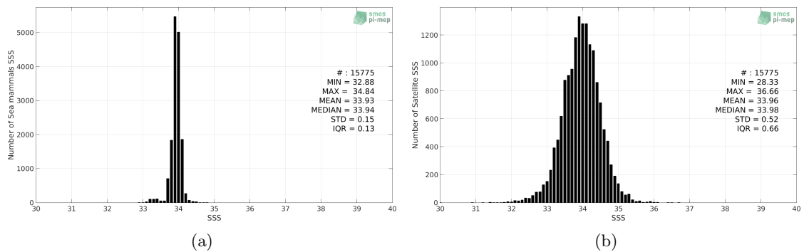
Figure 2: Histograms of SSS from Sea mammals (a) and SMAP-L3-RSS-V4-8DAY-RUNNING (b) considering all match-up pairs per bins of 0.1 over the Roaring Forties and Furious Fifties Pi-MEP region and for the full satellite product period.
