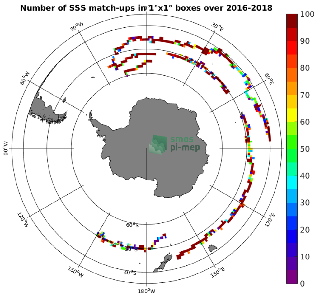
Figure 3: Number of SSS match-ups between Surface drifters SSS and the SMAP-L3-RSS-V4-8DAY-RUNNING SSS product for the Roaring Forties and Furious Fifties Pi-MEP region over 1°x1° boxes and for the full satellite product period.
