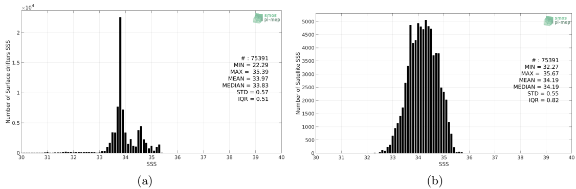
Figure 2: Histograms of SSS from Surface drifters (a) and SMAP-L3-RSS-V4-8DAY-RUNNING (b) considering all match-up pairs per bins of 0.1 over the Roaring Forties and Furious Fifties Pi-MEP region and for the full satellite product period.
