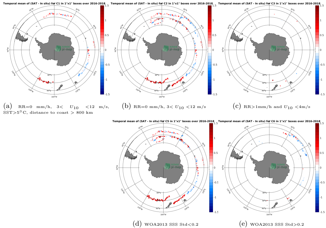
Figure 11: Temporal mean gridded over spatial boxes of size 1^{\circ}\times 1^{\circ} of \Delta\text{SSS} (SMAP-L3-RSS-V4-8DAY-RUNNING - Surface drifters) for 5 different subdatasets corresponding to:RR=0 mm/h, 3 < U_{10} < 12 m/s, SST >5^{\circ}\text{C} , distance to coast > 800 km (a), RR=0 mm/h, 3 < U_{10} < 12 m/s (b), RR >1 mm/h and U_{10} < 4 m/s (c), WOA2013 SSS Std <0.2 (d), WOA2013 SSS Std >0.2 (e).
