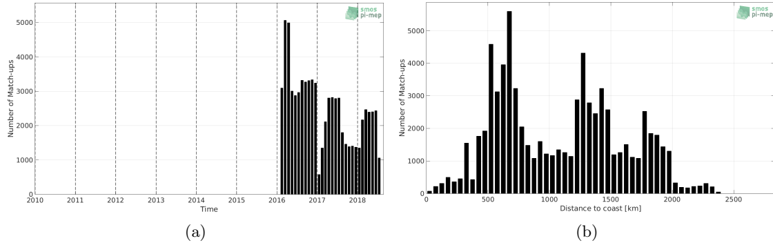
Figure 1: Number of match-ups between Surface drifters and SMAP-L3-RSS-V4-8DAY-RUNNING SSS as a function of time (a) and as function of the distance to coast (b) over the Roaring Forties and Furious Fifties Pi-MEP region and for the full satellite product period.
