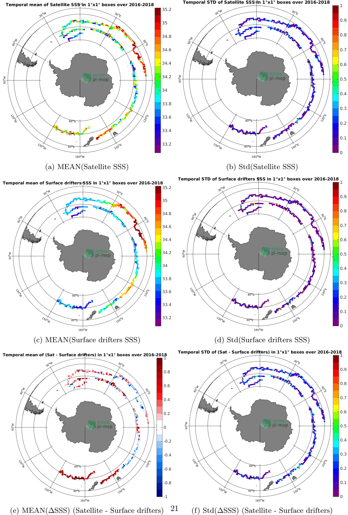
Figure 5: Temporal mean (left) and Std (right) of SSS from SMAP-L3-RSS-V4-8DAY-RUNNING (top), Surface drifters (middle), and of \Delta SSS (Satellite - Surface drifters). Only match-up pairs are used to generate these maps.
