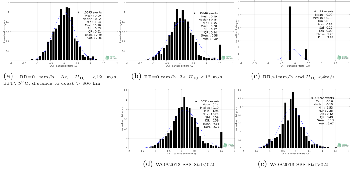
Figure 12: Normalized histogram of \Delta SSS (SMAP-L3-RSS-V4-8DAY-RUNNING - Surface drifters) for 5 different subdatasets corresponding to: RR=0 mm/h, 3 < U_{10} < 12 m/s, SST>5°C, distance to coast > 800 km (a), RR=0 mm/h, 3 < U_{10} < 12 m/s (b), RR>1mm/h and U_{10} < 4 m/s (c), WOA2013 SSS Std<0.2 (d), WOA2013 SSS Std>0.2 (e).
