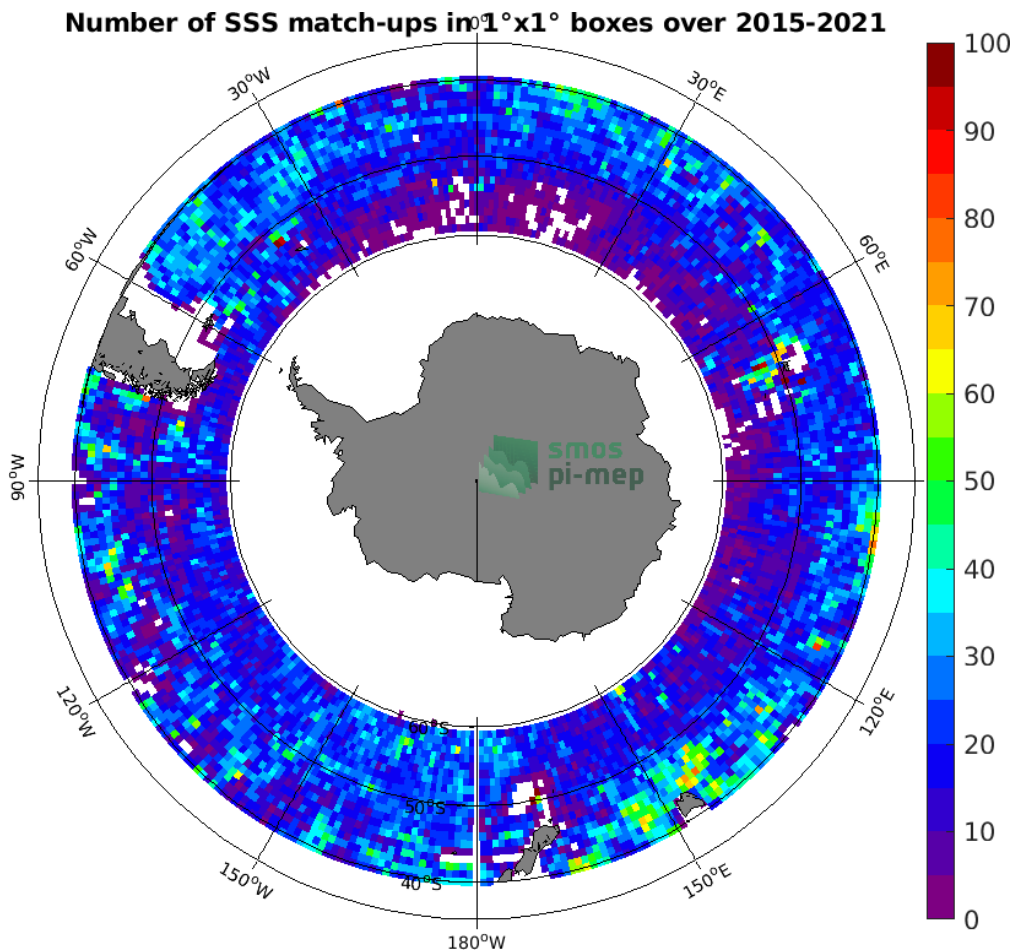
Figure 4: Number of SSS match-ups between Argo SSS and the SMAP SSS L3 v4 - 8-Day running (RSS) SSS product for the Roaring Forties and Furious Fifties Pi-MEP region over 1^\circ \times 1^\circ boxes and for the full satellite product period.
