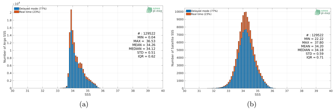
Figure 2: Histograms of SSS from Argo (a) and SMAP SSS L3 v4 - 8-Day running (RSS) (b) considering all match-up pairs per bins of 0.1 over the Roaring Forties and Furious Fifties Pi-MEP region and for the full satellite product period.
