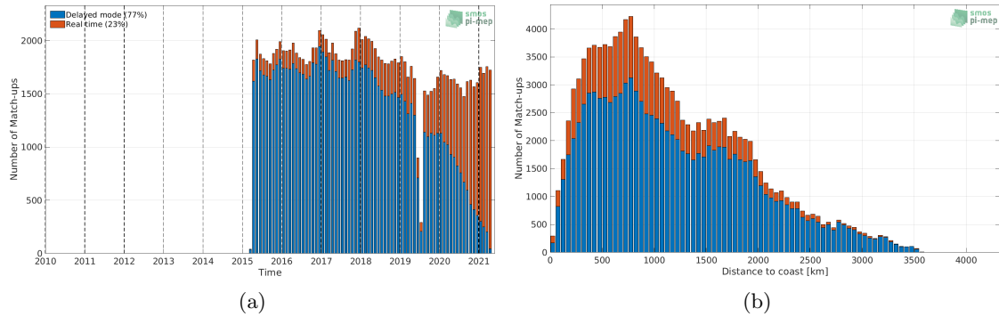
Figure 1: Number of match-ups between Argo and SMAP SSS L3 v4 - 8-Day running (RSS) SSS as a function of time (a) and as function of the distance to coast (b) over the Roaring Forties and Furious Fifties Pi-MEP region and for the full satellite product period.
