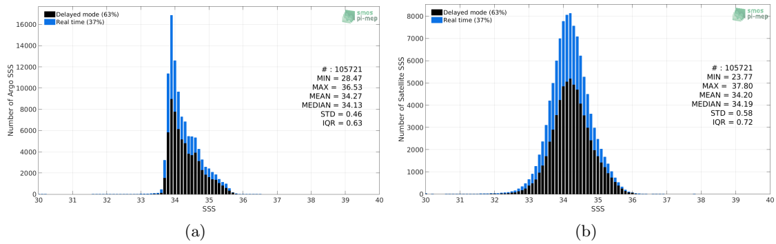
Figure 2: Histograms of SSS from Argo (a) and SMAP-L3-RSS-V4-8DAY-RUNNING (b) considering all match-up pairs per bins of 0.1 over the Roaring Forties and Furious Fifties Pi-MEP region and for the full satellite product period.
