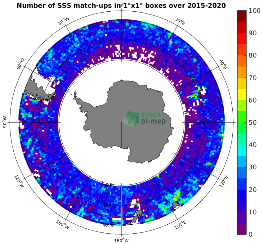
Figure 4: Number of SSS match-ups between Argo SSS and the SMAP-L3-RSS-V4-8DAY-RUNNING SSS product for the Roaring Forties and Furious Fifties Pi-MEP region over 1°x1° boxes and for the full satellite product period.
