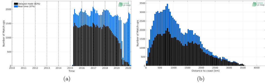
Figure 1: Number of match-ups between Argo and SMAP-L3-RSS-V4-8DAY-RUNNING SSS as a function of time (a) and as function of the distance to coast (b) over the Roaring Forties and Furious Fifties Pi-MEP region and for the full satellite product period.
