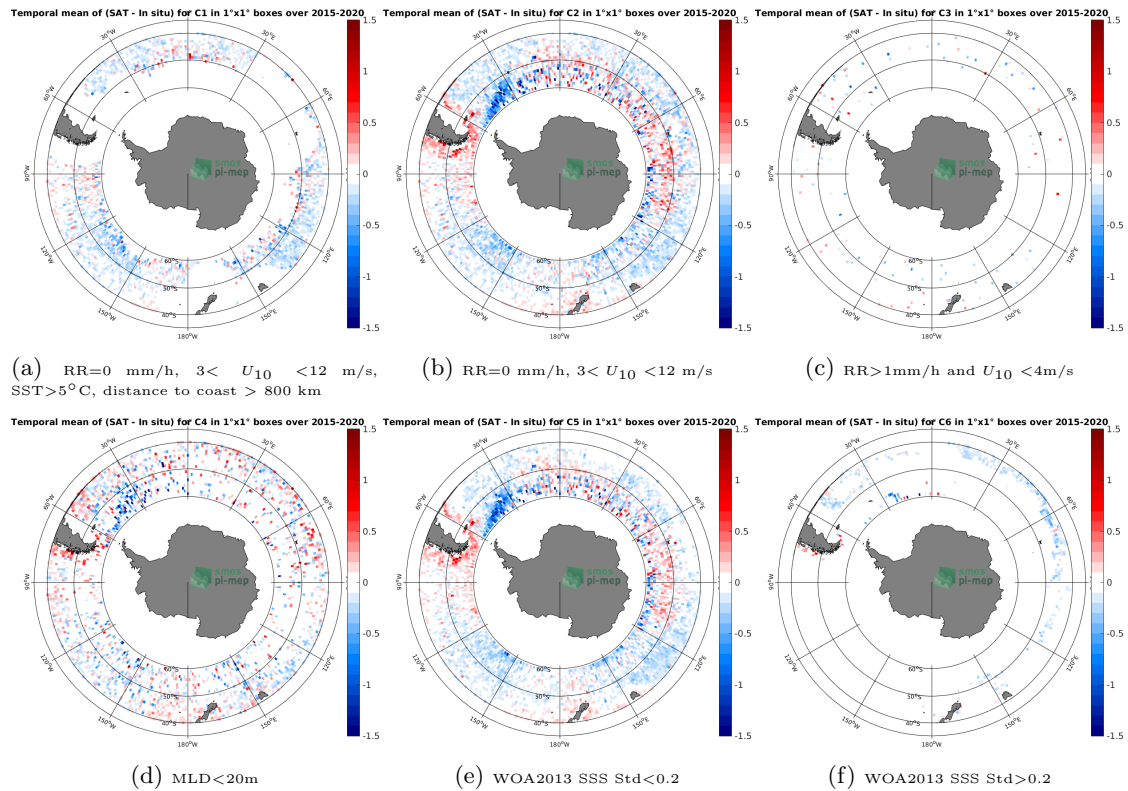
Figure 12: Temporal mean gridded over spatial boxes of size 1^{\circ}\times 1^{\circ} of \Delta\text{SSS} (SMAP-L3-RSS-V4-8DAY-RUNNING - Argo) for 6 different subdatasets corresponding to:RR=0 mm/h, 3 < U_{10} < 12 m/s, SST >5^{\circ}\text{C} , distance to coast > 800 km (a), RR=0 mm/h, 3 < U_{10} < 12 m/s (b), RR >1 mm/h and U_{10} < 4 m/s (c),MLD <20\text{m} (d),WOA2013 SSS Std <0.2 (e),WOA2013 SSS Std >0.2 (f).
