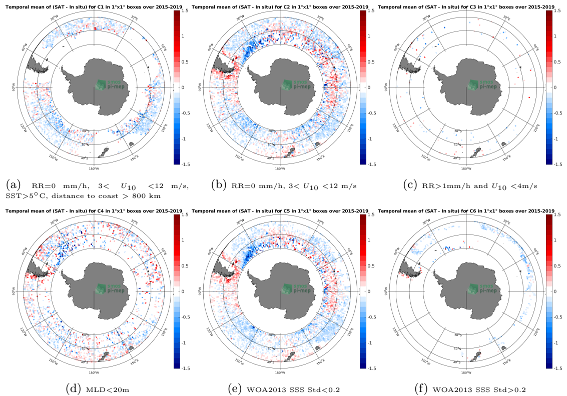
Figure 12: Temporal mean gridded over spatial boxes of size 1°x1° of \Delta SSS (SMAP-L3-RSS-V4-8DAY-RUNNING - Argo) for 6 different subdatasets corresponding to:RR=0 mm/h, 3 < U_{10} < 12 m/s, SST > 5°C, distance to coast > 800 km (a), RR=0 mm/h, 3 < U_{10} < 12 m/s (b), RR > 1mm/h and U_{10} < 4m/s (c),MLD < 20m (d),WOA2013 SSS Std < 0.2 (e),WOA2013 SSS Std > 0.2 (f).
