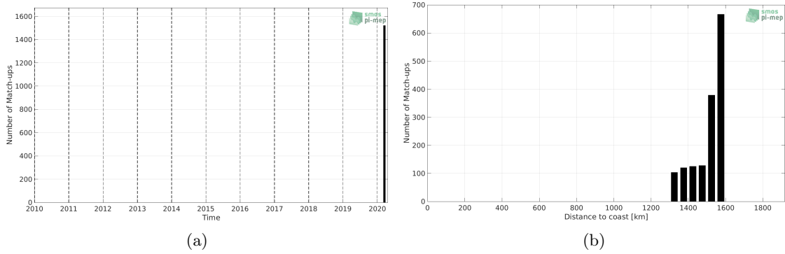
Figure 1: Number of match-ups between TSG (SAMOS) and SMAP SSS L3 v4 - Monthly (RSS) SSS as a function of time (a) and as function of the distance to coast (b) over the Roaring Forties and Furious Fifties Pi-MEP region and for the full satellite product period.
