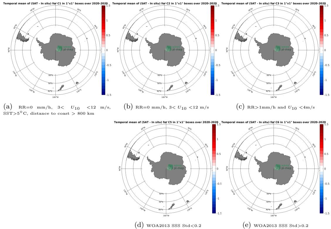
Figure 12: Temporal mean gridded over spatial boxes of size 1^{\circ}\times 1^{\circ} of \Delta\text{SSS} (SMAP SSS L3 v4 - Monthly (RSS) - TSG (SAMOS)) for 5 different subdatasets corresponding to:RR=0 mm/h, 3 < U_{10} < 12 m/s, SST > 5^{\circ}\text{C} , distance to coast > 800 km (a), RR=0 mm/h, 3 < U_{10} < 12 m/s (b), RR > 1 mm/h and U_{10} < 4 m/s (c), WOA2013 SSS Std < 0.2 (d), WOA2013 SSS Std > 0.2 (e).
