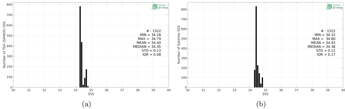
Figure 2: Histograms of SSS from TSG (SAMOS) (a) and SMAP SSS L3 v4 - Monthly (RSS) (b) considering all match-up pairs per bins of 0.1 over the Roaring Forties and Furious Fifties Pi-MEP region and for the full satellite product period.
