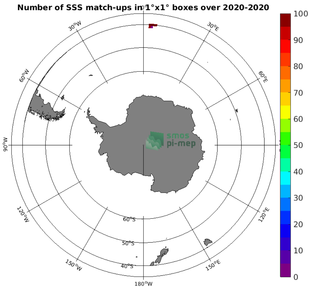
Figure 4: Number of SSS match-ups between TSG (SAMOS) SSS and the SMAP SSS L3 v4 - Monthly (RSS) SSS product for the Roaring Forties and Furious Fifties Pi-MEP region over 1°x1° boxes and for the full satellite product period.
