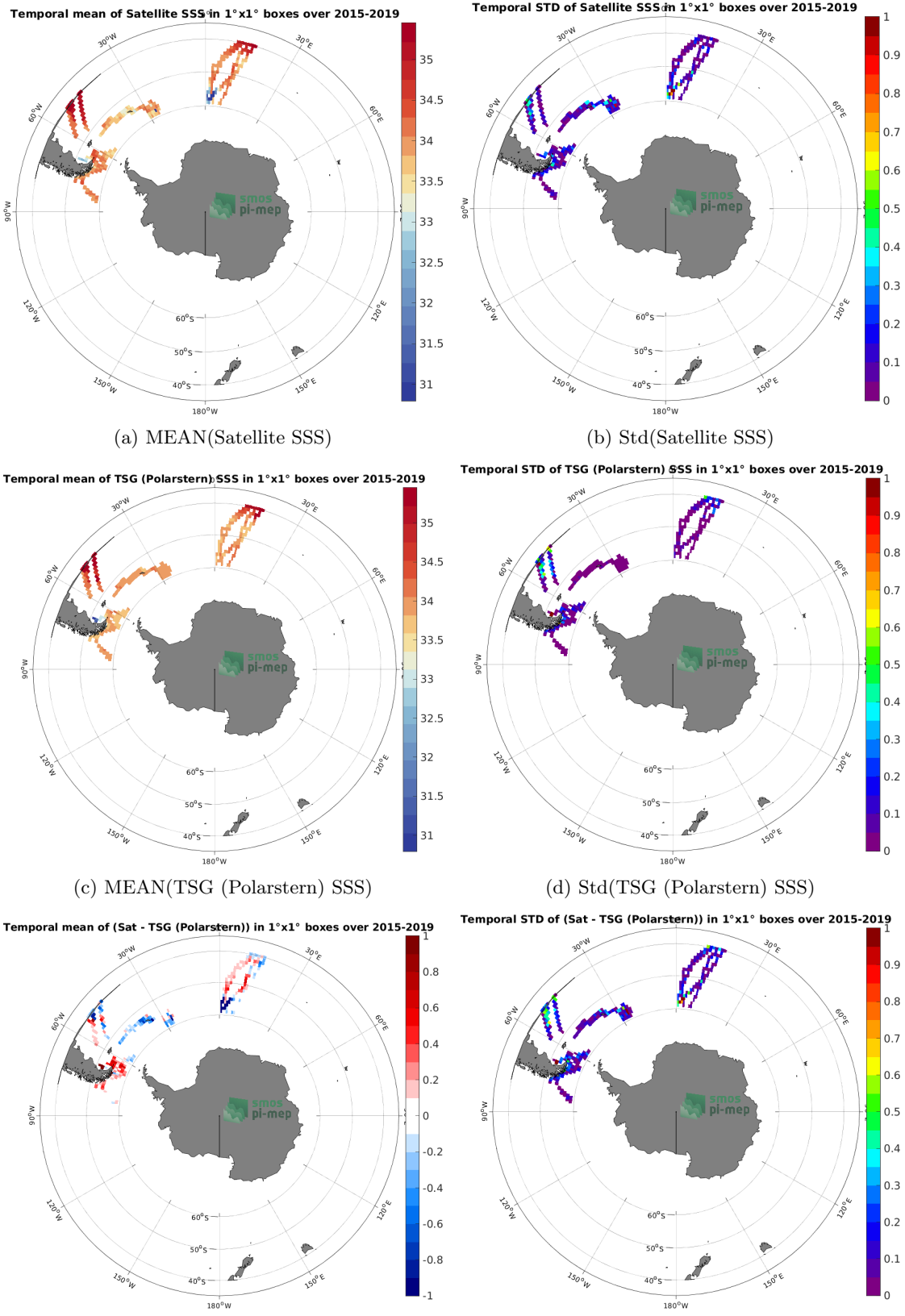
Figure 6: Temporal mean (left) and Std (right) of SSS from SMAP SSS L3 v4 - Monthly (RSS) (top), TSG (Polarstern) (middle), and of \Delta SSS (Satellite - TSG (Polarstern)). Only match-up pairs are used to generate these maps.
