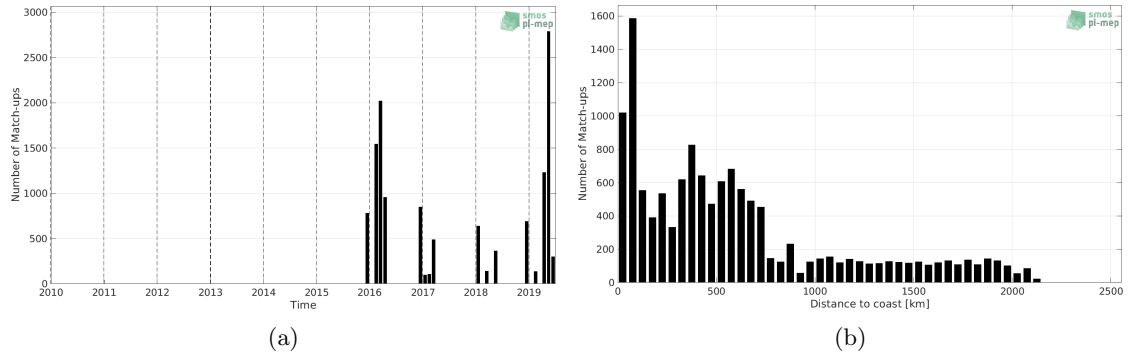
Figure 1: Number of match-ups between TSG (Polarstern) and SMAP SSS L3 v4 - Monthly (RSS) SSS as a function of time (a) and as function of the distance to coast (b) over the Roaring Forties and Furious Fifties Pi-MEP region and for the full satellite product period.
