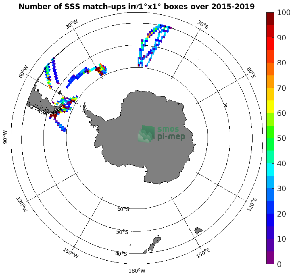
Figure 4: Number of SSS match-ups between TSG (Polarstern) SSS and the SMAP SSS L3 v4 - Monthly (RSS) SSS product for the Roaring Forties and Furious Fifties Pi-MEP region over 1^\circ \times 1^\circ boxes and for the full satellite product period.
