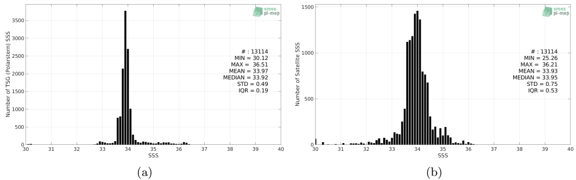
Figure 2: Histograms of SSS from TSG (Polarstern) (a) and SMAP SSS L3 v4 - Monthly (RSS) (b) considering all match-up pairs per bins of 0.1 over the Roaring Forties and Furious Fifties Pi-MEP region and for the full satellite product period.
