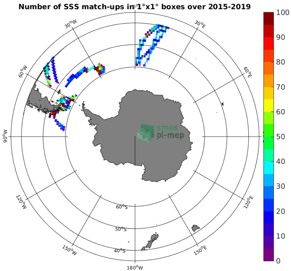
Figure 4: Number of SSS match-ups between TSG-POLARSTERN SSS and the SMAP-L3-RSS-V4-MONTHLY SSS product for the Roaring Forties and Furious Fifties Pi-MEP region over 1^\circ \times 1^\circ boxes and for the full satellite product period.
