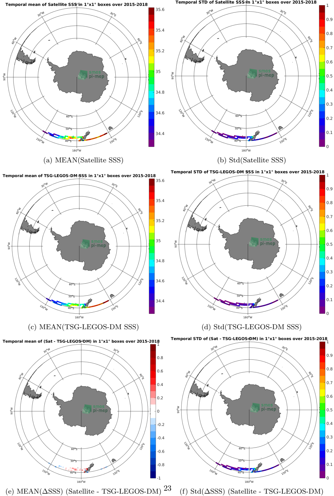
Figure 6: Temporal mean (left) and Std (right) of SSS from SMAP-L3-RSS-V4-MONTHLY (top), TSG-LEGOS-DM (middle), and of \Delta SSS (Satellite - TSG-LEGOS-DM). Only match-up pairs are used to generate these maps.
