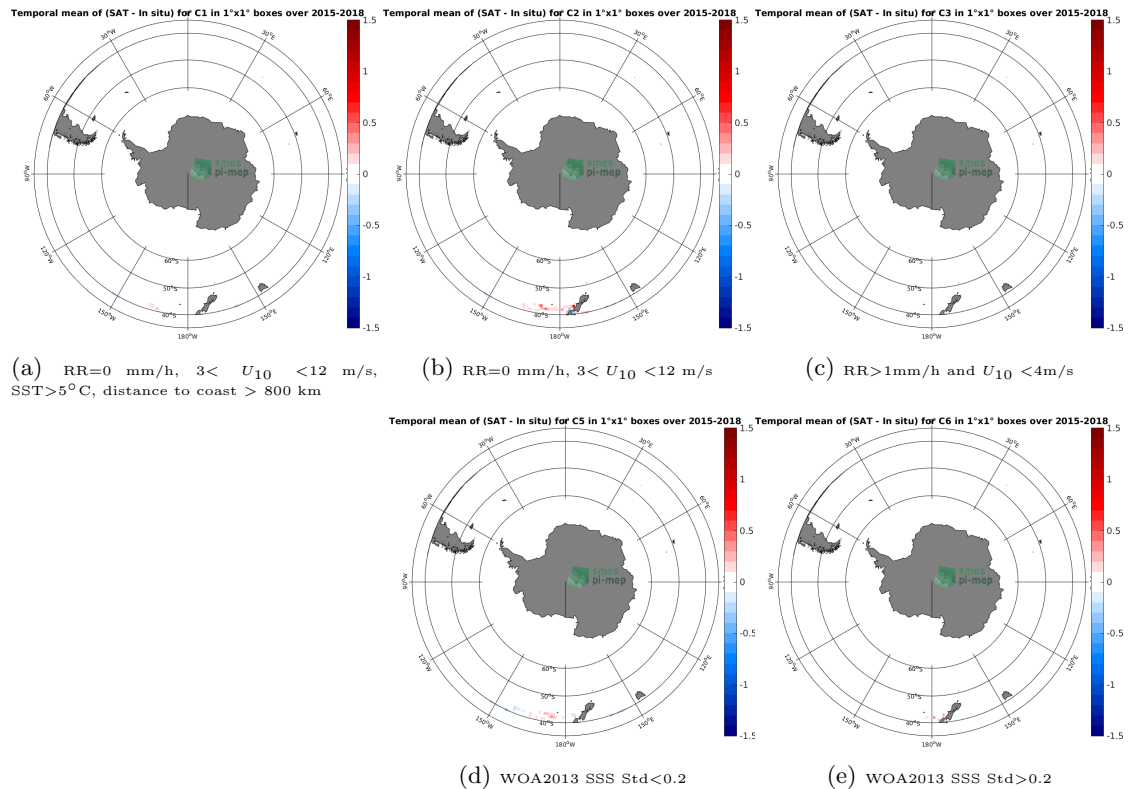
Figure 12: Temporal mean gridded over spatial boxes of size 1^\circ \times 1^\circ of \Delta SSS (SMAP-L3-RSS-V4-MONTHLY - TSG-LEGOS-DM) for 5 different subdatasets corresponding to:RR=0 mm/h, 3 < U_{10} < 12 m/s, SST >5^\circ C, distance to coast > 800 km (a), RR=0 mm/h, 3 < U_{10} < 12 m/s (b), RR >1 mm/h and U_{10} < 4 m/s (c), WOA2013 SSS Std <0.2 (d), WOA2013 SSS Std >0.2 (e).
