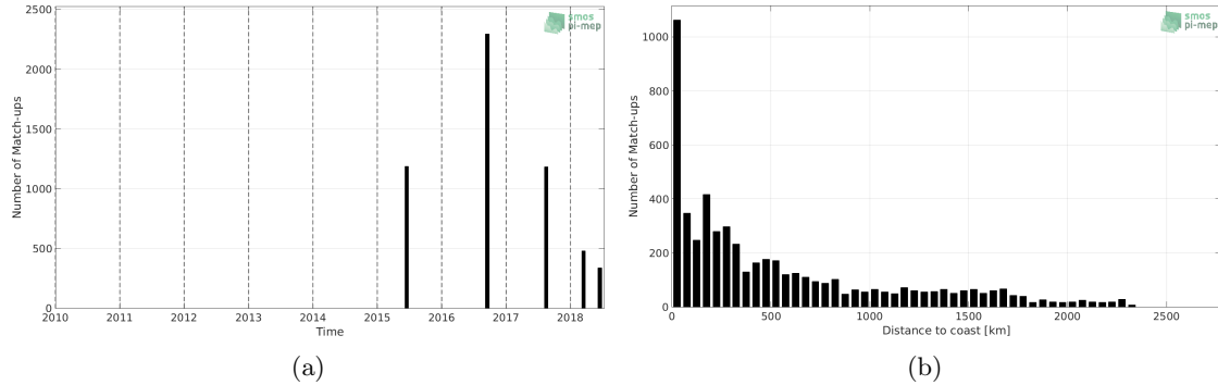
Figure 1: Number of match-ups between TSG-LEGOS-DM and SMAP-L3-RSS-V4-MONTHLY SSS as a function of time (a) and as function of the distance to coast (b) over the Roaring Forties and Furious Fifties Pi-MEP region and for the full satellite product period.
