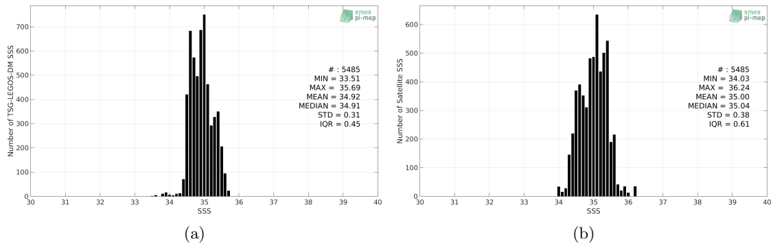
Figure 2: Histograms of SSS from TSG-LEGOS-DM (a) and SMAP-L3-RSS-V4-MONTHLY (b) considering all match-up pairs per bins of 0.1 over the Roaring Forties and Furious Fifties Pi-MEP region and for the full satellite product period.
