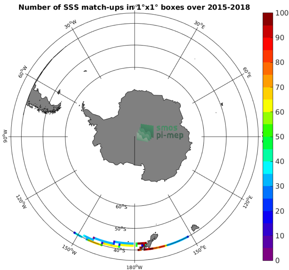
Figure 4: Number of SSS match-ups between TSG-LEGOS-DM SSS and the SMAP-L3-RSS-V4-MONTHLY SSS product for the Roaring Forties and Furious Fifties Pi-MEP region over 1°x1° boxes and for the full satellite product period.
