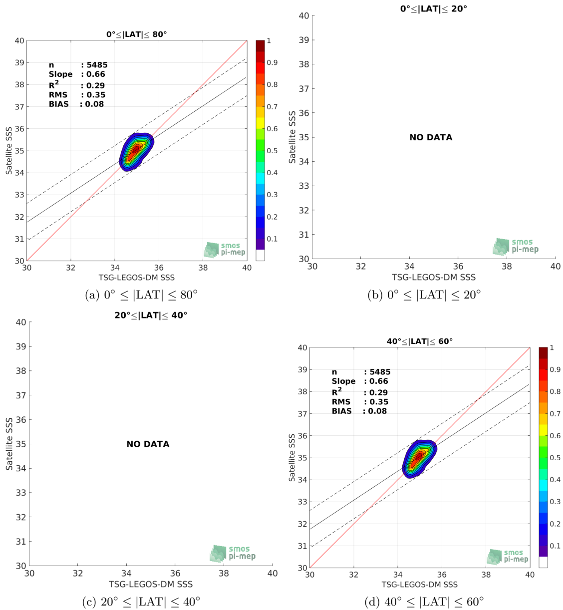
Figure 9: Contour maps of the concentration of SMAP-L3-RSS-V4-MONTHLY SSS (y-axis) versus TSG-LEGOS-DM SSS (x-axis) at match-up pairs for different latitude bands. For each plot, the red line shows x=y . The black thin and dashed lines indicate a linear fit through the data cloud and the \pm 95\% confidence levels, respectively. The number match-up pairs n , the slope and R^2 coefficient of the linear fit, the root mean square (RMS) and the mean bias between satellite and in situ data are indicated for each latitude band in each plots.
