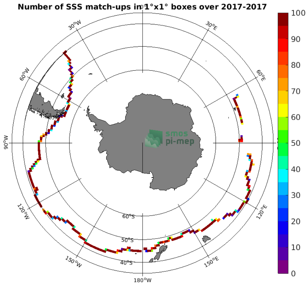
Figure 4: Number of SSS match-ups between TSG (GOSUD-Sailing-ship) SSS and the SMAP SSS L3 v4 - Monthly (RSS) SSS product for the Roaring Forties and Furious Fifties Pi-MEP region over 1°x1° boxes and for the full satellite product period.
