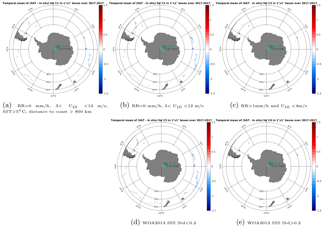
Figure 12: Temporal mean gridded over spatial boxes of size 1°x1° of \Delta SSS (SMAP-L3-RSS-V4-MONTHLY - TSG-GOSUD-Sailing-ship) for 5 different subdatasets corresponding to:RR=0 mm/h, 3 < U_{10} < 12 m/s, SST>5°C, distance to coast > 800 km (a), RR=0 mm/h, 3 < U_{10} < 12 m/s (b), RR>1mm/h and U_{10} < 4 m/s (c), WOA2013 SSS Std<0.2 (d), WOA2013 SSS Std>0.2 (e).
