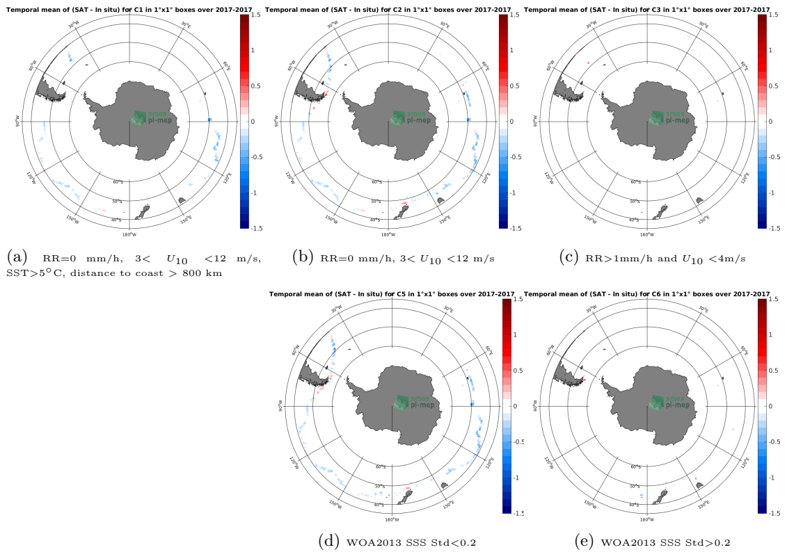
Figure 12: Temporal mean gridded over spatial boxes of size 1°x1° of ΔSSS (SMAP-L3-RSS-V4-MONTHLY - TSG-GOSUD-Sailing-ship) for 5 different subdatasets corresponding to:RR=0 mm/h, 3 < U_{10} < 12 m/s, SST>5°C, distance to coast > 800 km (a), RR=0 mm/h, 3 < U_{10} < 12 m/s (b), RR>1mm/h and U_{10} < 4 m/s (c), WOA2013 SSS Std<0.2 (d), WOA2013 SSS Std>0.2 (e).
