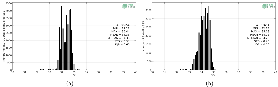
Figure 2: Histograms of SSS from TSG-GOSUD-Sailing-ship (a) and SMAP-L3-RSS-V4-MONTHLY (b) considering all match-up pairs per bins of 0.1 over the Roaring Forties and Furious Fifties Pi-MEP region and for the full satellite product period.
