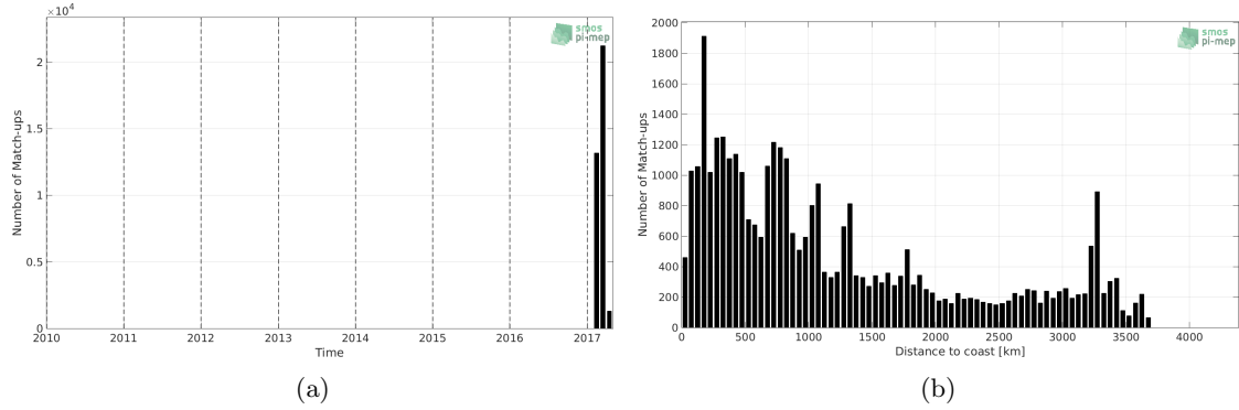
Figure 1: Number of match-ups between TSG-GOSUD-Sailing-ship and SMAP-L3-RSS-V4-MONTHLY SSS as a function of time (a) and as function of the distance to coast (b) over the Roaring Forties and Furious Fifties Pi-MEP region and for the full satellite product period.
