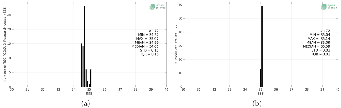
Figure 2: Histograms of SSS from TSG (GOSUD-Research-vessel) (a) and SMAP SSS L3 v4 - Monthly (RSS) (b) considering all match-up pairs per bins of 0.1 over the Roaring Forties and Furious Fifties Pi-MEP region and for the full satellite product period.
