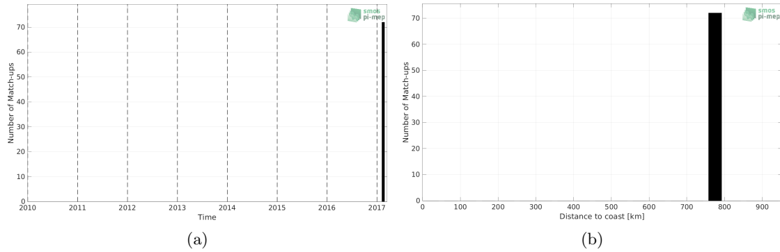
Figure 1: Number of match-ups between TSG (GOSUD-Research-vessel) and SMAP SSS L3 v4 - Monthly (RSS) SSS as a function of time (a) and as function of the distance to coast (b) over the Roaring Forties and Furious Fifties Pi-MEP region and for the full satellite product period.
