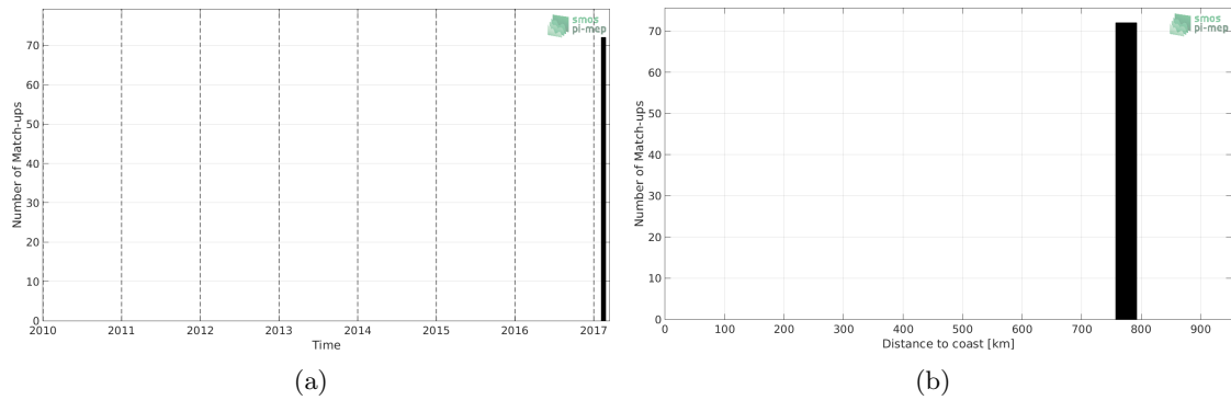
Figure 1: Number of match-ups between TSG (GOSUD-Research-vessel) and SMAP SSS L3 v4 - Monthly (RSS) SSS as a function of time (a) and as function of the distance to coast (b) over the Roaring Forties and Furious Fifties Pi-MEP region and for the full satellite product period.
