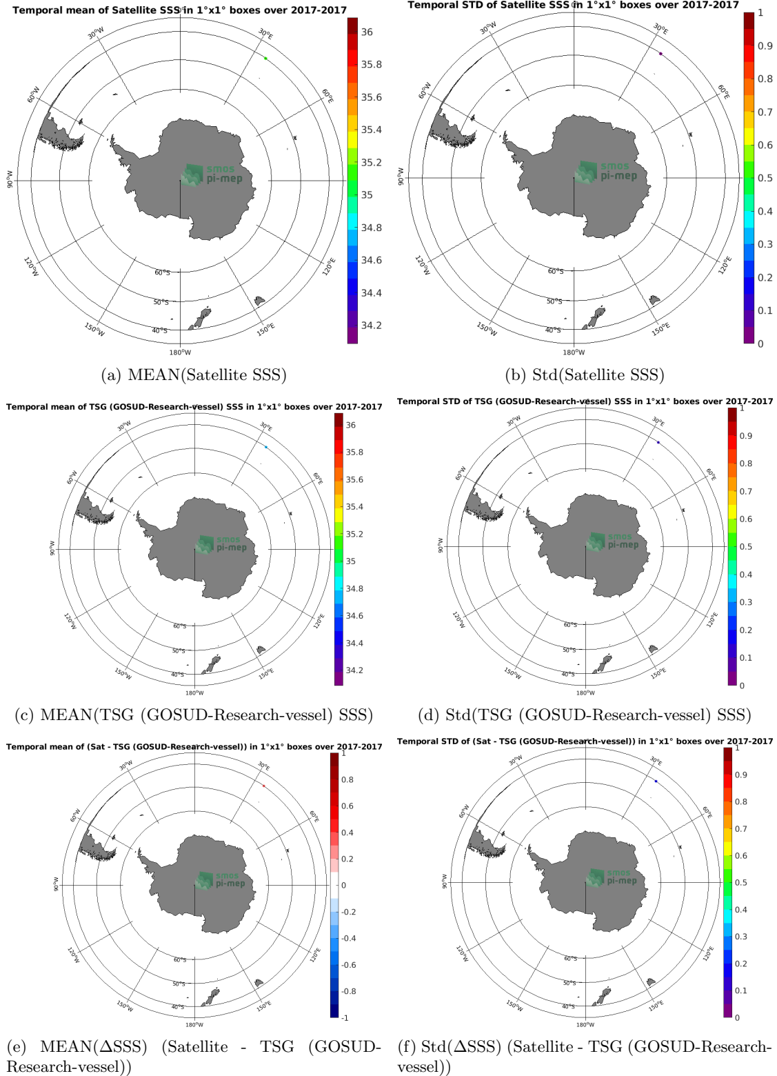
Figure 6: Temporal mean (left) and Std (right) of SSS from SMAP SSS L3 v4 - Monthly (RSS) (top), TSG (GOSUD-Research-vessel) (middle), and of \Delta SSS (Satellite - TSG (GOSUD-Research-vessel)). Only match-up pairs are used to generate these maps.
