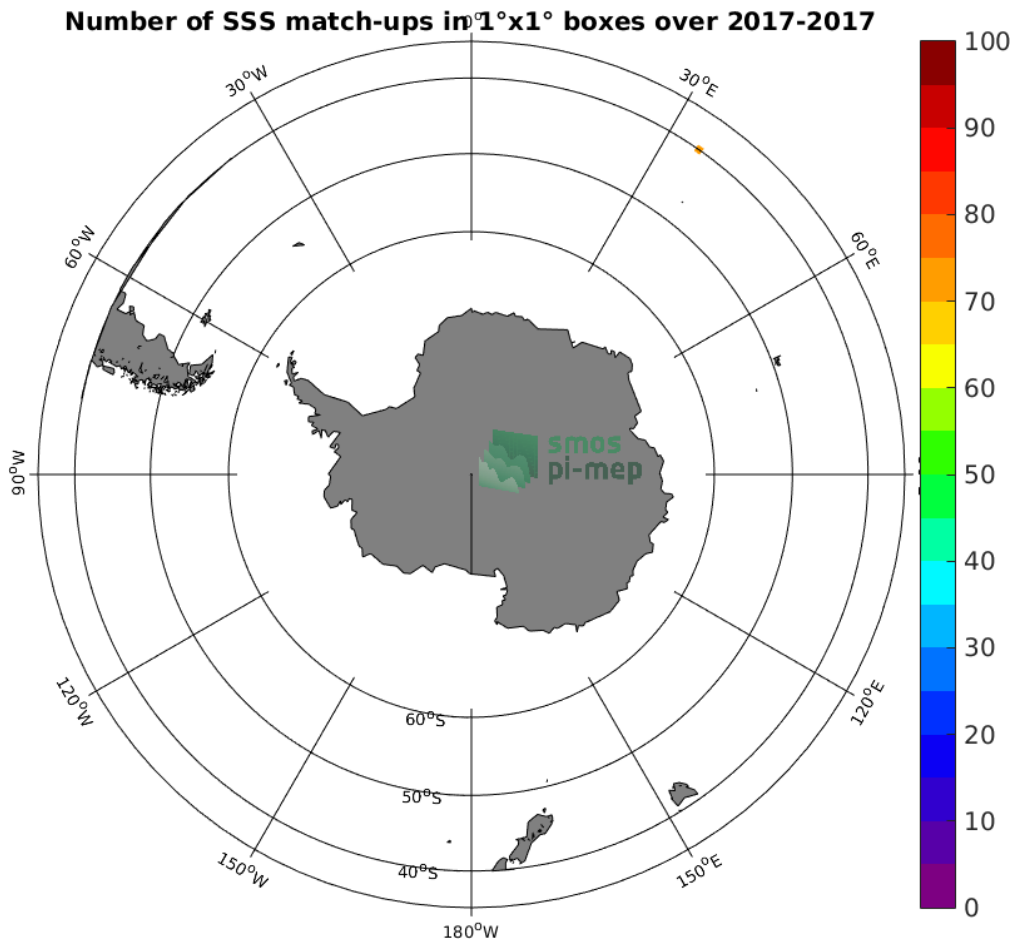
Figure 4: Number of SSS match-ups between TSG-GOSUD-Research-vessel SSS and the SMAP-L3-RSS-V4-MONTHLY SSS product for the Roaring Forties and Furious Fifties Pi-MEP region over 1°x1° boxes and for the full satellite product period.
