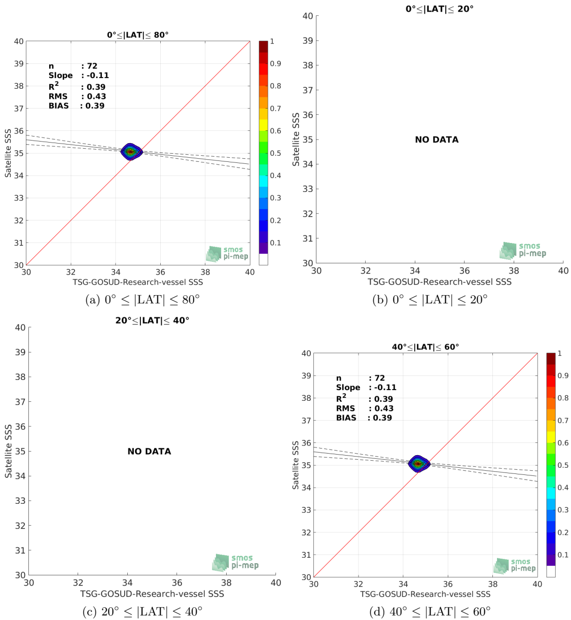
Figure 9: Contour maps of the concentration of SMAP-L3-RSS-V4-MONTHLY SSS (y-axis) versus TSG-GOSUD-Research-vessel SSS (x-axis) at match-up pairs for different latitude bands. For each plot, the red line shows x=y . The black thin and dashed lines indicate a linear fit through the data cloud and the \pm 95\% confidence levels, respectively. The number match-up pairs n , the slope and R^2 coefficient of the linear fit, the root mean square (RMS) and the mean bias between satellite and in situ data are indicated for each latitude band in each plots.
