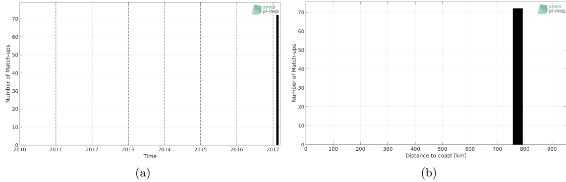
Figure 1: Number of match-ups between TSG-GOSUD-Research-vessel and SMAP-L3-RSS-V4-MONTHLY SSS as a function of time (a) and as function of the distance to coast (b) over the Roaring Forties and Furious Fifties Pi-MEP region and for the full satellite product period.
