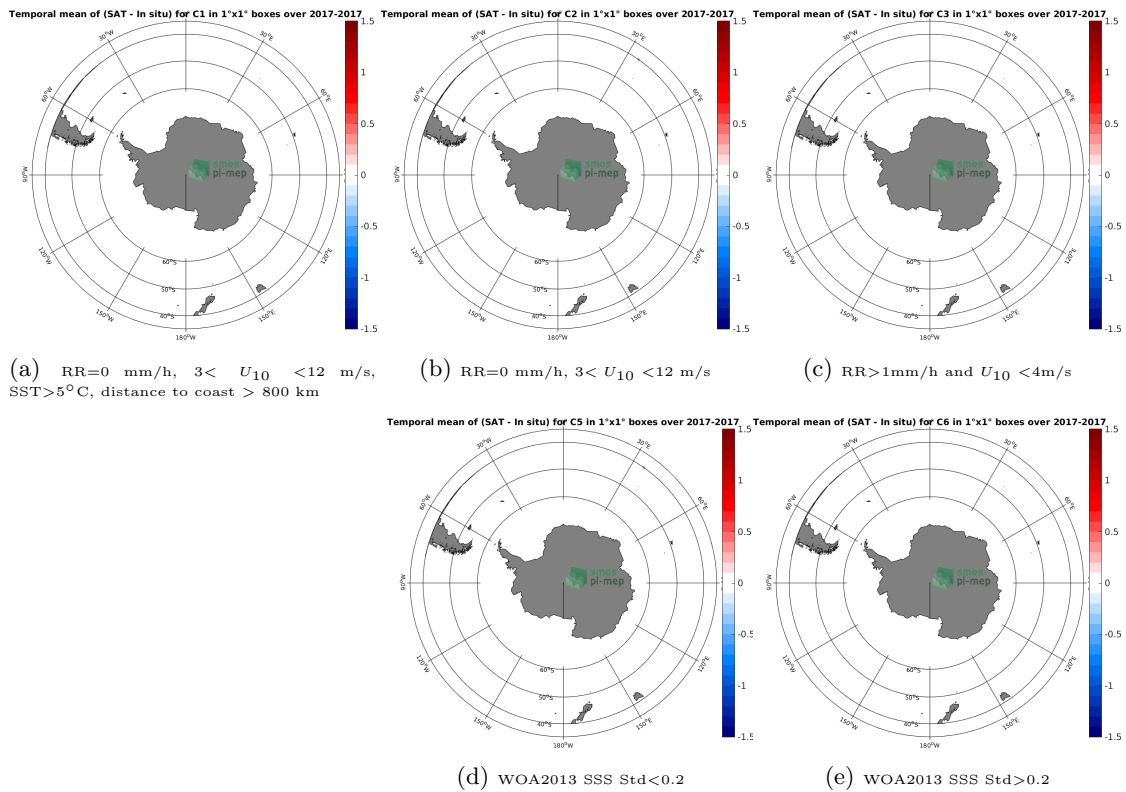
Figure 12: Temporal mean gridded over spatial boxes of size 1°x1° of \Delta SSS (SMAP-L3-RSS-V4-MONTHLY - TSG-GOSUD-Research-vessel) for 5 different subdatasets corresponding to:RR=0 mm/h, 3 < U_{10} < 12 m/s, SST>5°C, distance to coast > 800 km (a), RR=0 mm/h, 3 < U_{10} < 12 m/s (b), RR>1mm/h and U_{10} < 4 m/s (c), WOA2013 SSS Std<0.2 (d), WOA2013 SSS Std>0.2 (e).
