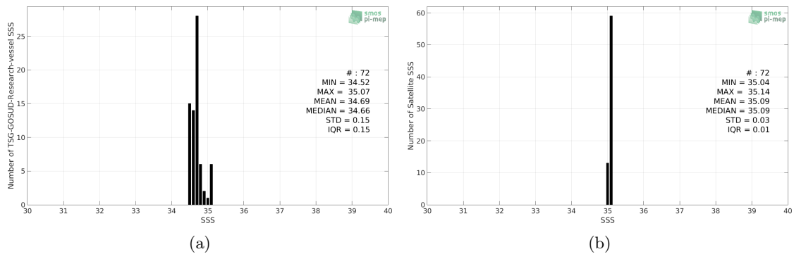
Figure 2: Histograms of SSS from TSG-GOSUD-Research-vessel (a) and SMAP-L3-RSS-V4-MONTHLY (b) considering all match-up pairs per bins of 0.1 over the Roaring Forties and Furious Fifties Pi-MEP region and for the full satellite product period.
