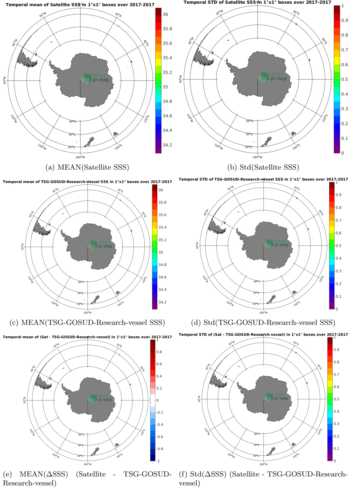
Figure 6: Temporal mean (left) and Std (right) of SSS from SMAP-L3-RSS-V4-MONTHLY (top), TSG-GOSUD-Research-vessel (middle), and of \Delta SSS (Satellite - TSG-GOSUD-Research-vessel). Only match-up pairs are used to generate these maps.
