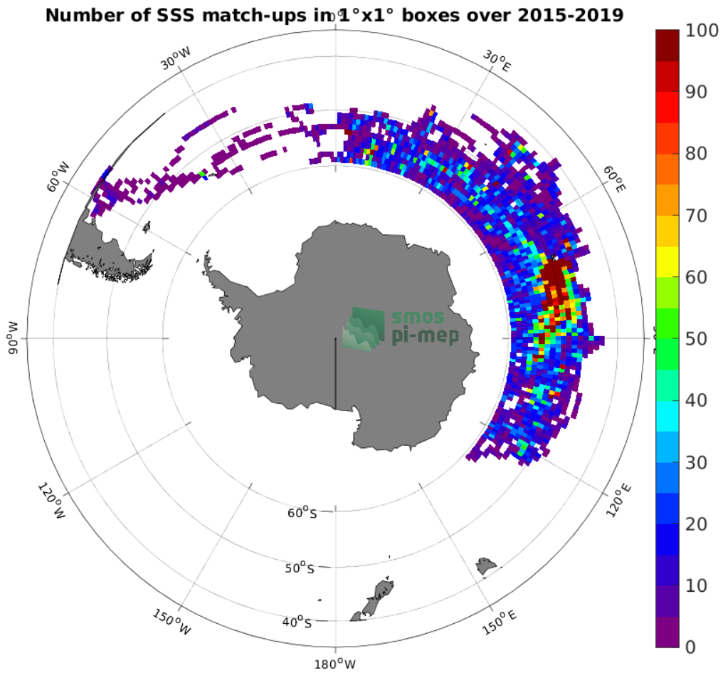
Figure 4: Number of SSS match-ups between Marine mammals SSS and the SMAP SSS L3 v4 - Monthly (RSS) SSS product for the Roaring Forties and Furious Fifties Pi-MEP region over 1^\circ \times 1^\circ boxes and for the full satellite product period.
