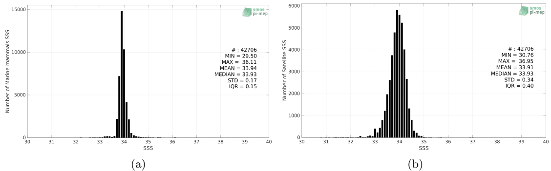
Figure 2: Histograms of SSS from Marine mammals (a) and SMAP SSS L3 v4 - Monthly (RSS) (b) considering all match-up pairs per bins of 0.1 over the Roaring Forties and Furious Fifties Pi-MEP region and for the full satellite product period.
