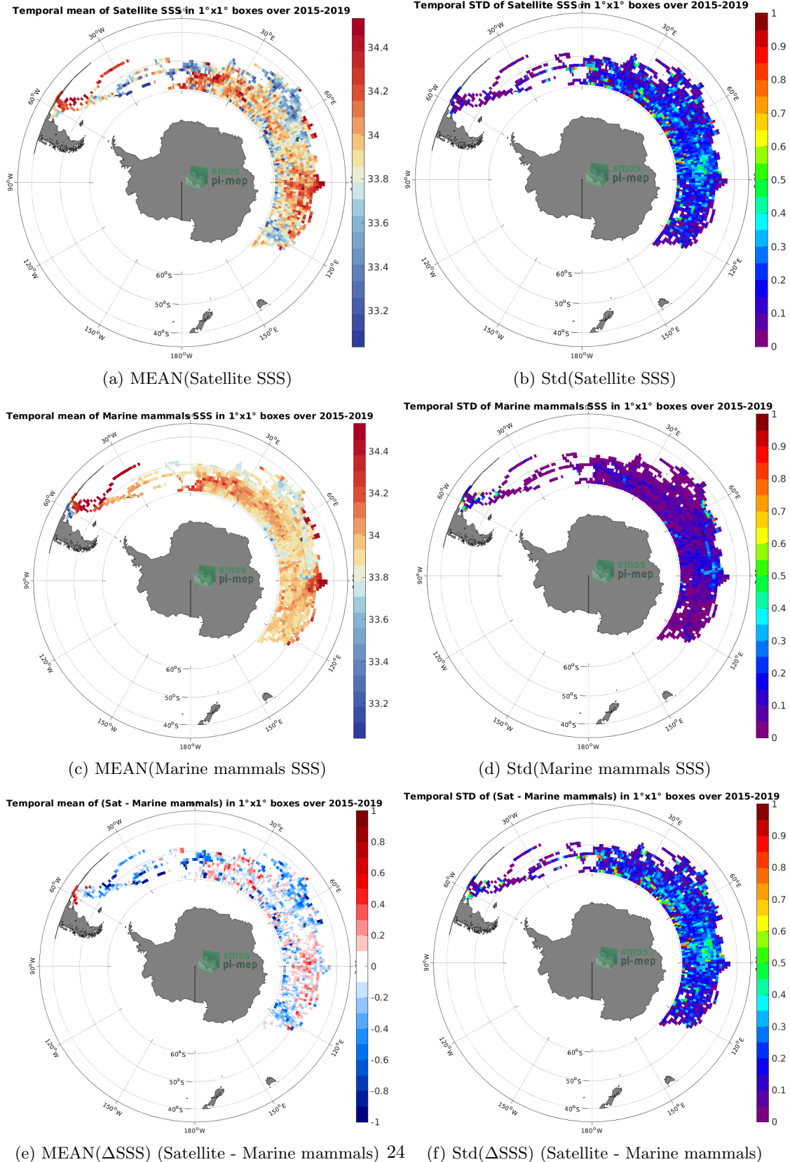
Figure 6: Temporal mean (left) and Std (right) of SSS from SMAP SSS L3 v4 - Monthly (RSS) (top), Marine mammals (middle), and of \Delta SSS (Satellite - Marine mammals). Only match-up pairs are used to generate these maps.
