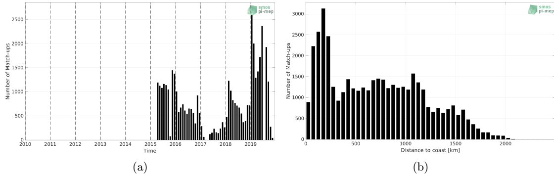
Figure 1: Number of match-ups between Marine mammals and SMAP SSS L3 v4 - Monthly (RSS) SSS as a function of time (a) and as function of the distance to coast (b) over the Roaring Forties and Furious Fifties Pi-MEP region and for the full satellite product period.
