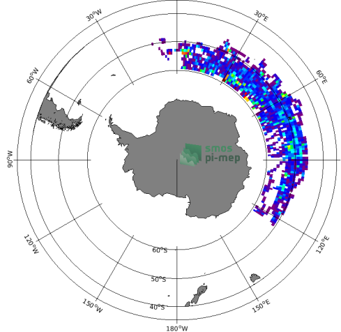
(f) Std( \Delta SSS) (Satellite - Sea mammals)
