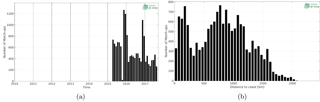
Figure 1: Number of match-ups between Sea mammals and SMAP SSS L3 v4 - Monthly (RSS) SSS as a function of time (a) and as function of the distance to coast (b) over the Roaring Forties and Furious Fifties Pi-MEP region and for the full satellite product period.
