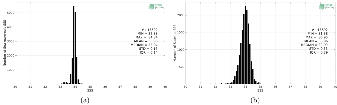
Figure 2: Histograms of SSS from Sea mammals (a) and SMAP SSS L3 v4 - Monthly (RSS) (b) considering all match-up pairs per bins of 0.1 over the Roaring Forties and Furious Fifties Pi-MEP region and for the full satellite product period.
