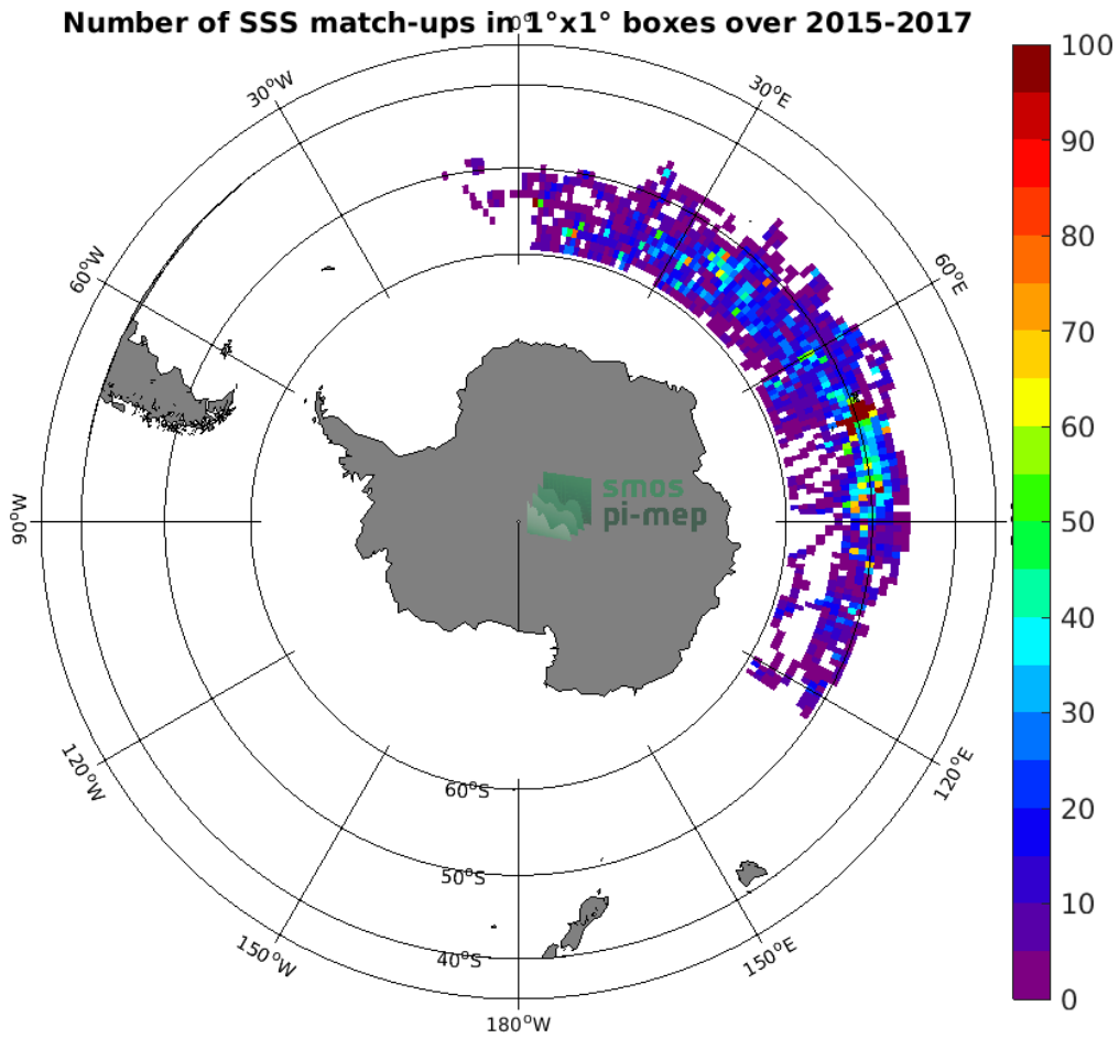
Figure 4: Number of SSS match-ups between Sea mammals SSS and the SMAP SSS L3 v4 - Monthly (RSS) SSS product for the Roaring Forties and Furious Fifties Pi-MEP region over 1°x1° boxes and for the full satellite product period.
