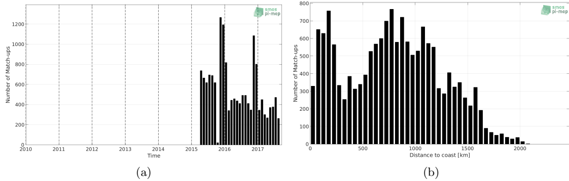
Figure 1: Number of match-ups between Sea mammals and SMAP-L3-RSS-V4-MONTHLY SSS as a function of time (a) and as function of the distance to coast (b) over the Roaring Forties and Furious Fifties Pi-MEP region and for the full satellite product period.
