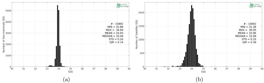
Figure 2: Histograms of SSS from Sea mammals (a) and SMAP-L3-RSS-V4-MONTHLY (b) considering all match-up pairs per bins of 0.1 over the Roaring Forties and Furious Fifties Pi-MEP region and for the full satellite product period.
