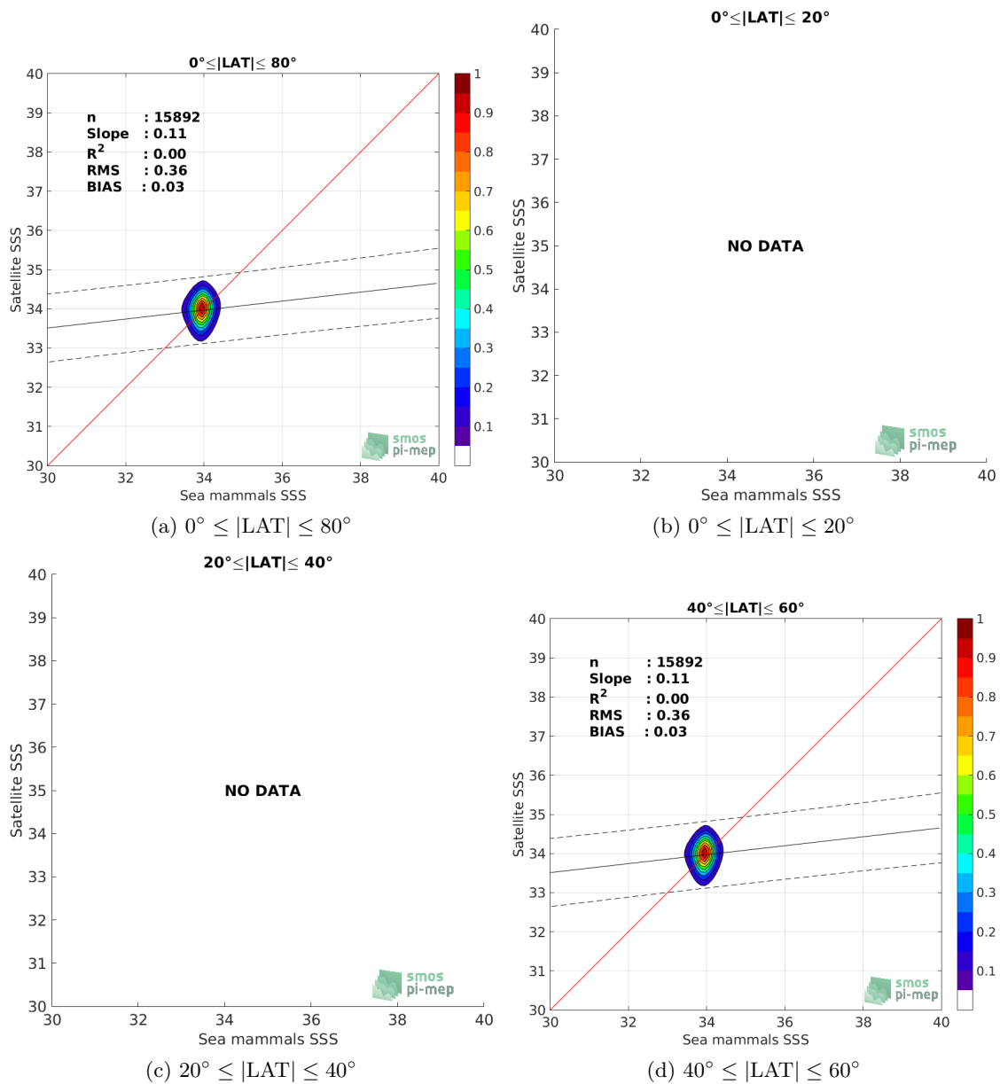
Figure 9: Contour maps of the concentration of SMAP-L3-RSS-V4-MONTHLY SSS (y-axis) versus Sea mammals SSS (x-axis) at match-up pairs for different latitude bands. For each plot, the red line shows x=y . The black thin and dashed lines indicate a linear fit through the data cloud and the \pm 95\% confidence levels, respectively. The number match-up pairs n , the slope and R^2 coefficient of the linear fit, the root mean square (RMS) and the mean bias between satellite and in situ data are indicated for each latitude band in each plots.
