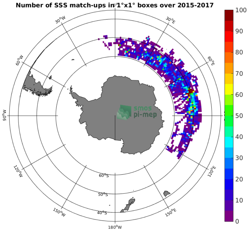
Figure 4: Number of SSS match-ups between Sea mammals SSS and the SMAP-L3-RSS-V4-MONTHLY SSS product for the Roaring Forties and Furious Fifties Pi-MEP region over 1^{\circ} \times 1^{\circ} boxes and for the full satellite product period.
