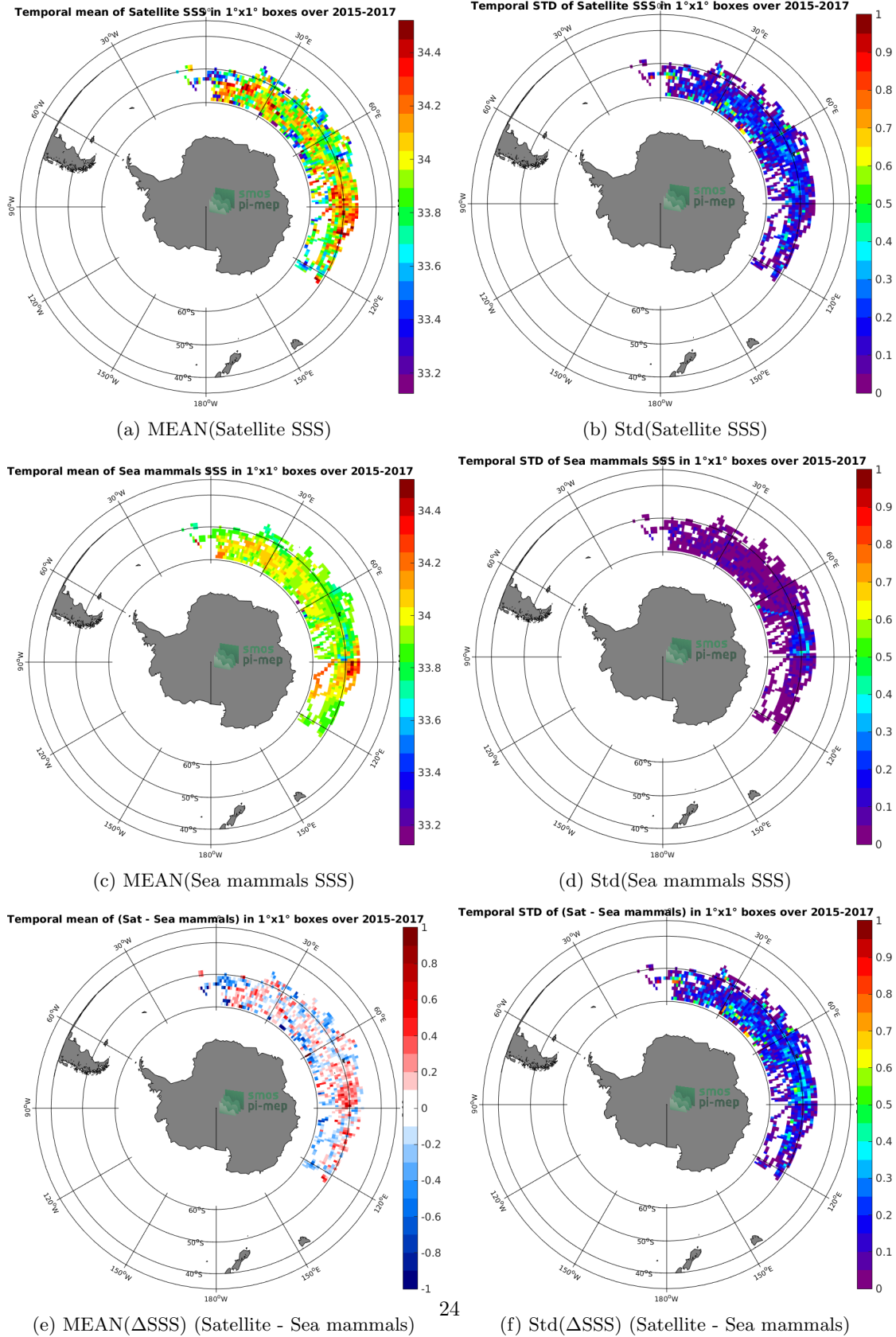
Figure 6: Temporal mean (left) and Std (right) of SSS from SMAP-L3-RSS-V4-MONTHLY (top), Sea mammals (middle), and of \Delta SSS (Satellite - Sea mammals). Only match-up pairs are used to generate these maps.
