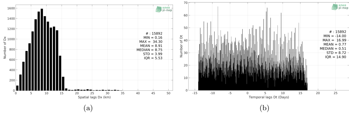
Figure 5: Histograms of the spatial (a) and temporal (b) lags between the time of the Sea mammals measurements and the date of the corresponding SMAP-L3-RSS-V4-MONTHLY SSS product.
