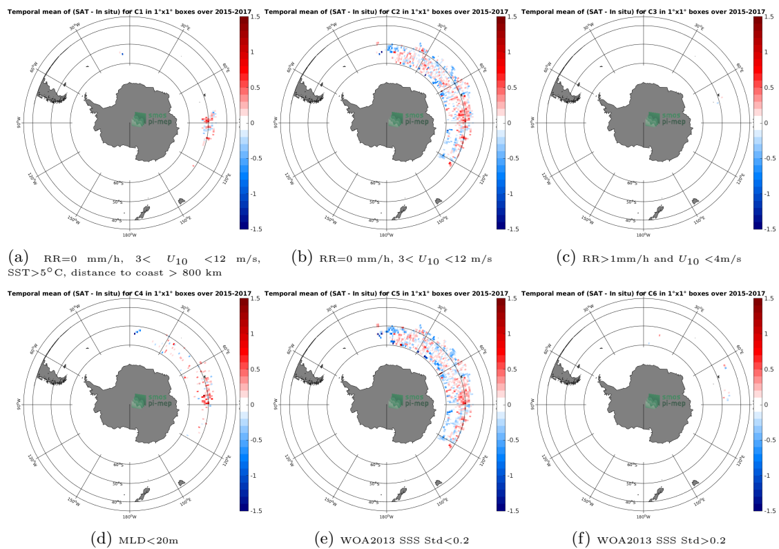
Figure 12: Temporal mean gridded over spatial boxes of size 1^\circ \times 1^\circ of \Delta SSS (SMAP-L3-RSS-V4-MONTHLY - Sea mammals) for 6 different subdatasets corresponding to:RR=0 mm/h, 3 < U_{10} < 12 m/s, SST > 5^\circ\text{C} , distance to coast > 800 km (a), RR=0 mm/h, 3 < U_{10} < 12 m/s (b), RR > 1 mm/h and U_{10} < 4 m/s (c),MLD < 20 m (d),WOA2013 SSS Std < 0.2 (e),WOA2013 SSS Std > 0.2 (f).
