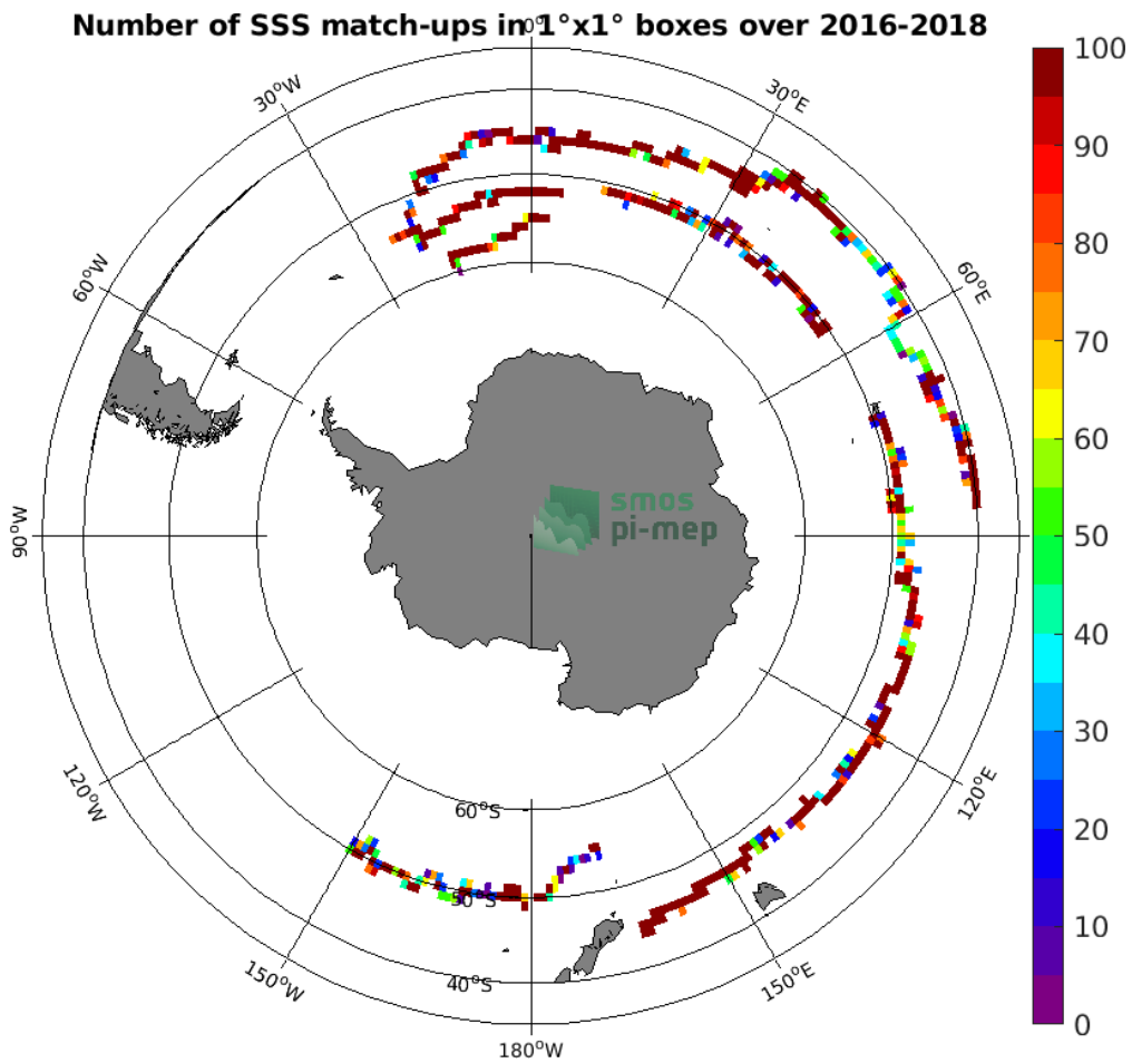
Figure 3: Number of SSS match-ups between Surface drifters SSS and the SMAP SSS L3 v4 - Monthly (RSS) SSS product for the Roaring Forties and Furious Fifties Pi-MEP region over 1^\circ \times 1^\circ boxes and for the full satellite product period.
