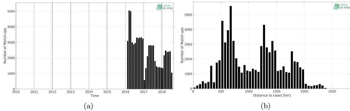
Figure 1: Number of match-ups between Surface drifters and SMAP SSS L3 v4 - Monthly (RSS) SSS as a function of time (a) and as function of the distance to coast (b) over the Roaring Forties and Furious Fifties Pi-MEP region and for the full satellite product period.
