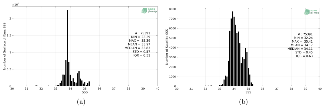
Figure 2: Histograms of SSS from Surface drifters (a) and SMAP SSS L3 v4 - Monthly (RSS) (b) considering all match-up pairs per bins of 0.1 over the Roaring Forties and Furious Fifties Pi-MEP region and for the full satellite product period.
