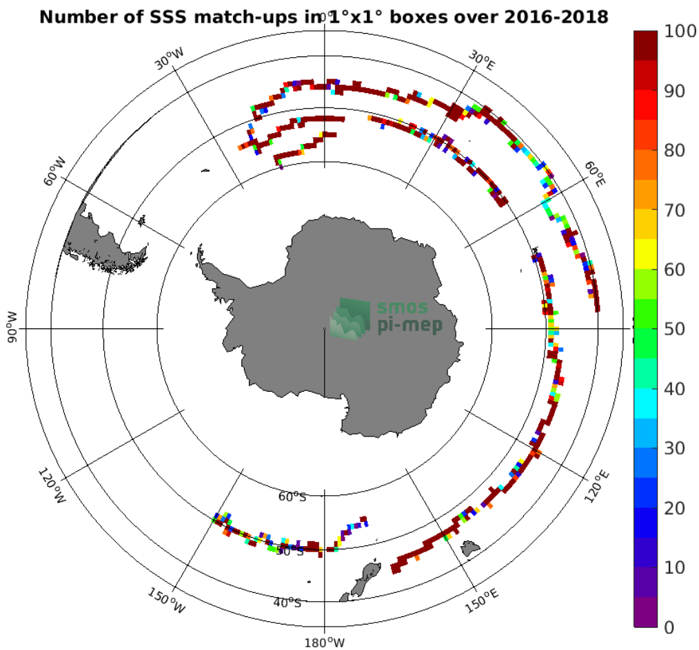
Figure 3: Number of SSS match-ups between Surface drifters SSS and the SMAP SSS L3 v4 - Monthly (RSS) SSS product for the Roaring Forties and Furious Fifties Pi-MEP region over 1°x1° boxes and for the full satellite product period.
