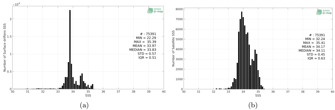
Figure 2: Histograms of SSS from Surface drifters (a) and SMAP-L3-RSS-V4-MONTHLY (b) considering all match-up pairs per bins of 0.1 over the Roaring Forties and Furious Fifties Pi-MEP region and for the full satellite product period.
