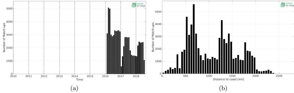
Figure 1: Number of match-ups between Surface drifters and SMAP-L3-RSS-V4-MONTHLY SSS as a function of time (a) and as function of the distance to coast (b) over the Roaring Forties and Furious Fifties Pi-MEP region and for the full satellite product period.
