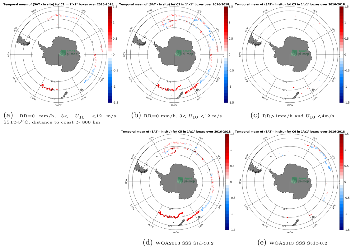
Figure 11: Temporal mean gridded over spatial boxes of size 1^{\circ}\times 1^{\circ} of \Delta\text{SSS} (SMAP-L3-RSS-V4-MONTHLY - Surface drifters) for 5 different subdatasets corresponding to: \text{RR}=0 mm/h, 3 < U_{10} < 12 m/s, \text{SST}>5^{\circ}\text{C} , distance to coast > 800 km (a), \text{RR}=0 mm/h, 3 < U_{10} < 12 m/s (b), \text{RR}>1\text{mm/h} and U_{10} < 4\text{m/s} (c), WOA2013 SSS Std < 0.2 (d), WOA2013 SSS Std > 0.2 (e).
