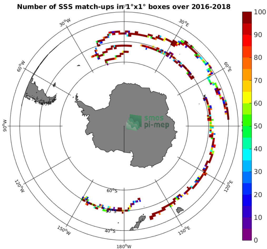
Figure 3: Number of SSS match-ups between Surface drifters SSS and the SMAP-L3-RSS-V4-MONTHLY SSS product for the Roaring Forties and Furious Fifties Pi-MEP region over 1°x1° boxes and for the full satellite product period.
