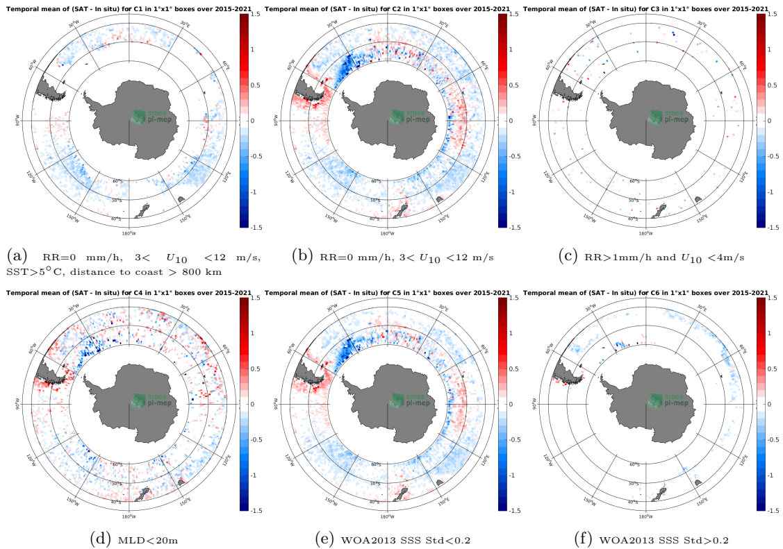
Figure 12: Temporal mean gridded over spatial boxes of size 1^{\circ}\times 1^{\circ} of \Delta\text{SSS} (SMAP SSS L3 v4 - Monthly (RSS) - Argo) for 6 different subdatasets corresponding to:RR=0 mm/h, 3 < U_{10} < 12 m/s, SST >5^{\circ}\text{C} , distance to coast > 800 km (a), RR=0 mm/h, 3 < U_{10} < 12 m/s (b), RR >1\text{mm/h} and U_{10} < 4\text{m/s} (c),MLD <20\text{m} (d),WOA2013 SSS Std <0.2 (e),WOA2013 SSS Std >0.2 (f).
