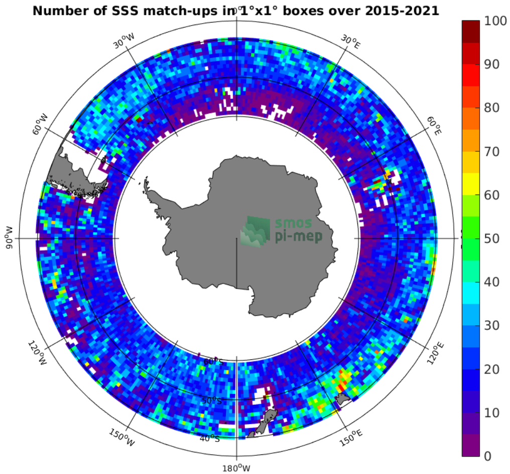
Figure 4: Number of SSS match-ups between Argo SSS and the SMAP SSS L3 v4 - Monthly (RSS) SSS product for the Roaring Forties and Furious Fifties Pi-MEP region over 1^\circ \times 1^\circ boxes and for the full satellite product period.
