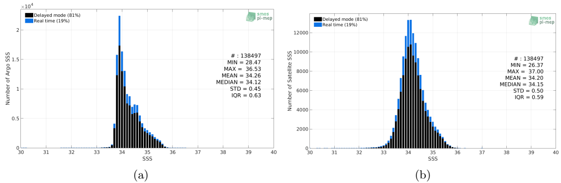
Figure 2: Histograms of SSS from Argo (a) and SMAP SSS L3 v4 - Monthly (RSS) (b) considering all match-up pairs per bins of 0.1 over the Roaring Forties and Furious Fifties Pi-MEP region and for the full satellite product period.
