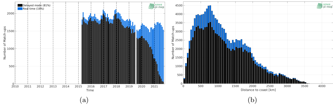
Figure 1: Number of match-ups between Argo and SMAP SSS L3 v4 - Monthly (RSS) SSS as a function of time (a) and as function of the distance to coast (b) over the Roaring Forties and Furious Fifties Pi-MEP region and for the full satellite product period.
