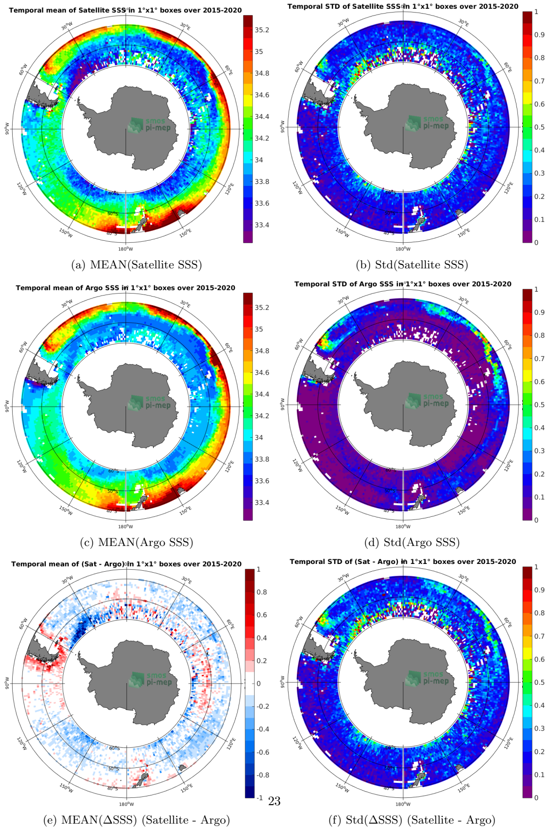
Figure 6: Temporal mean (left) and Std (right) of SSS from SMAP-L3-RSS-V4-MONTHLY (top), Argo (middle), and of \Delta SSS (Satellite - Argo). Only match-up pairs are used to generate these maps.
