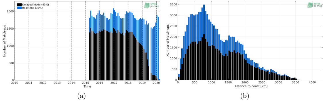
Figure 1: Number of match-ups between Argo and SMAP-L3-RSS-V4-MONTHLY SSS as a function of time (a) and as function of the distance to coast (b) over the Roaring Forties and Furious Fifties Pi-MEP region and for the full satellite product period.
