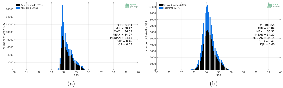
Figure 2: Histograms of SSS from Argo (a) and SMAP-L3-RSS-V4-MONTHLY (b) considering all match-up pairs per bins of 0.1 over the Roaring Forties and Furious Fifties Pi-MEP region and for the full satellite product period.
