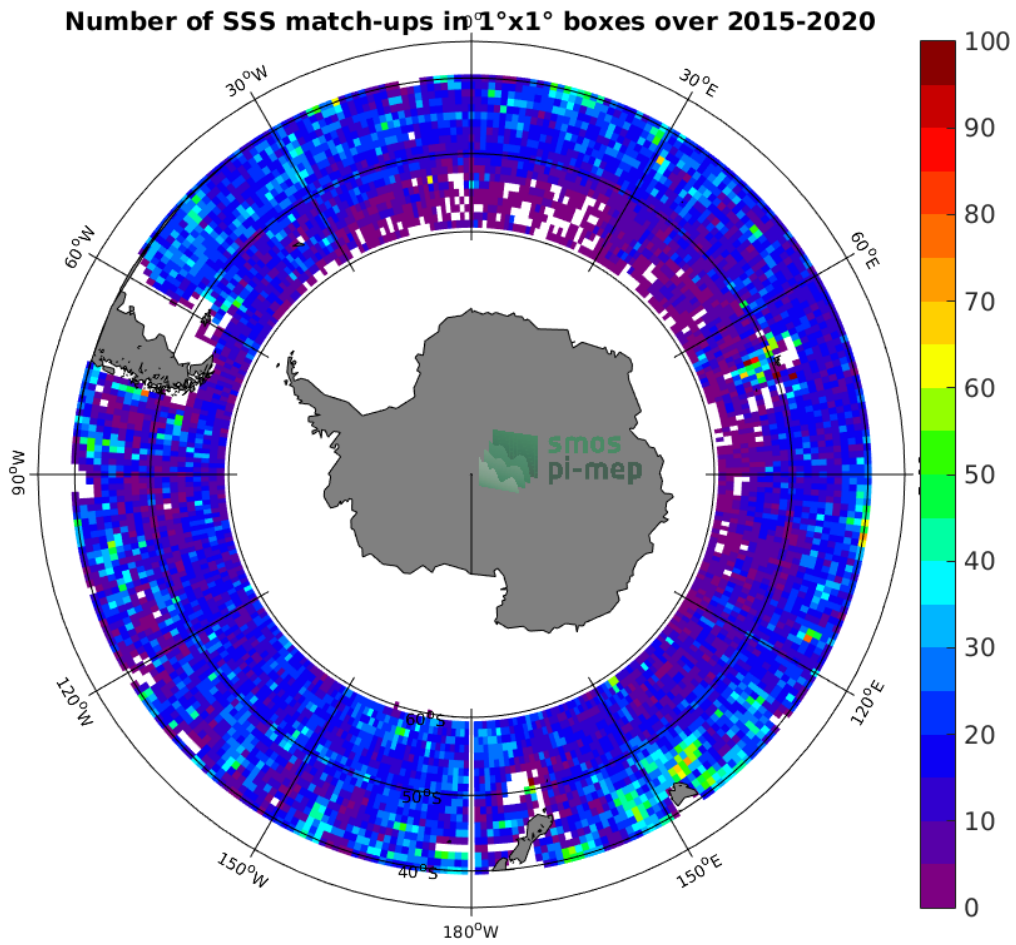
Figure 4: Number of SSS match-ups between Argo SSS and the SMAP-L3-RSS-V4-MONTHLY SSS product for the Roaring Forties and Furious Fifties Pi-MEP region over 1^\circ \times 1^\circ boxes and for the full satellite product period.
