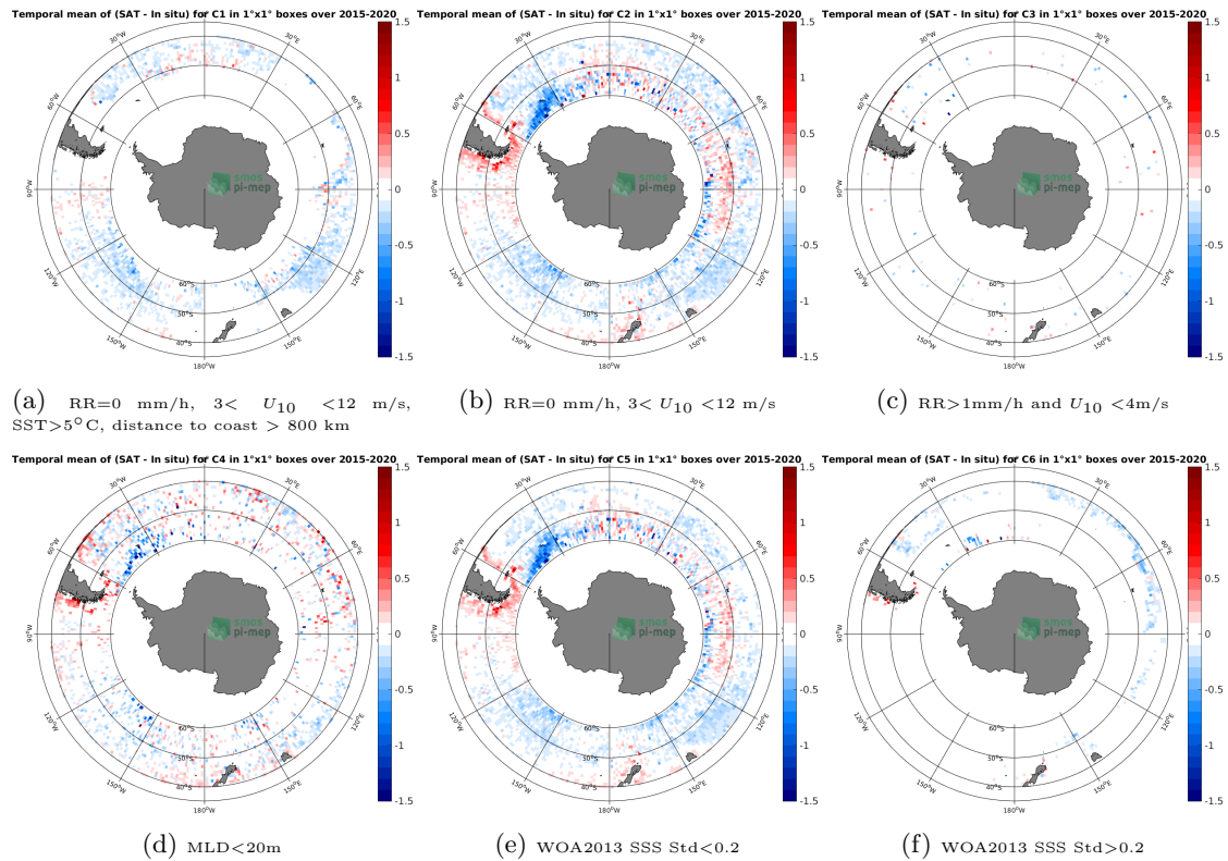
Figure 12: Temporal mean gridded over spatial boxes of size 1^{\circ}\times 1^{\circ} of \Delta\text{SSS} (SMAP-L3-RSS-V4-MONTHLY - Argo) for 6 different subdatasets corresponding to:RR=0 mm/h, 3 < U_{10} < 12 m/s, SST >5^{\circ}\text{C} , distance to coast > 800 km (a), RR=0 mm/h, 3 < U_{10} < 12 m/s (b), RR >1 mm/h and U_{10} < 4 m/s (c),MLD <20 m (d),WOA2013 SSS Std <0.2 (e),WOA2013 SSS Std >0.2 (f).
