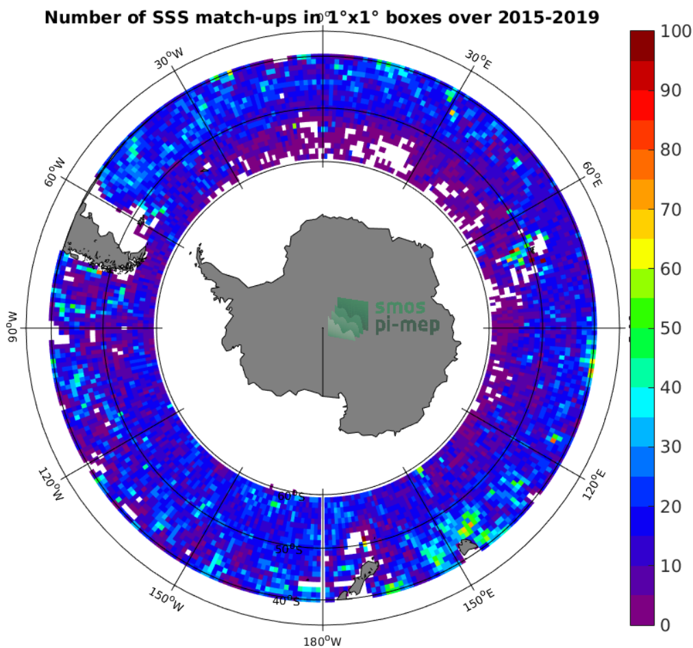
Figure 4: Number of SSS match-ups between Argo SSS and the SMAP-L3-RSS-V4-MONTHLY SSS product for the Roaring Forties and Furious Fifties Pi-MEP region over 1°x1° boxes and for the full satellite product period.
