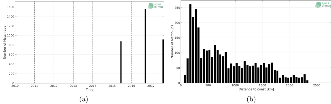
Figure 1: Number of match-ups between TSG-LEGOS-DM and SMAP-L3-RSS-V3-8DAY-RUNNING-70KM SSS as a function of time (a) and as function of the distance to coast (b) over the Roaring Forties and Furious Fifties Pi-MEP region and for the full satellite product period.
