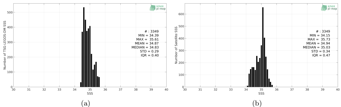
Figure 2: Histograms of SSS from TSG-LEGOS-DM (a) and SMAP-L3-RSS-V3-8DAY-RUNNING-70KM (b) considering all match-up pairs per bins of 0.1 over the Roaring Forties and Furious Fifties Pi-MEP region and for the full satellite product period.
