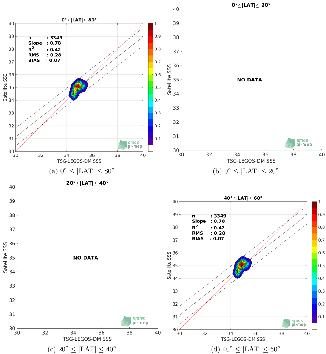
Figure 9: Contour maps of the concentration of SMAP-L3-RSS-V3-8DAY-RUNNING-70KM SSS (y-axis) versus TSG-LEGOS-DM SSS (x-axis) at match-up pairs for different latitude bands. For each plot, the red line shows x=y . The black thin and dashed lines indicate a linear fit through the data cloud and the \pm 95\% confidence levels, respectively. The number match-up pairs n , the slope and R^2 coefficient of the linear fit, the root mean square (RMS) and the mean bias between satellite and in situ data are indicated for each latitude band in each plots.
