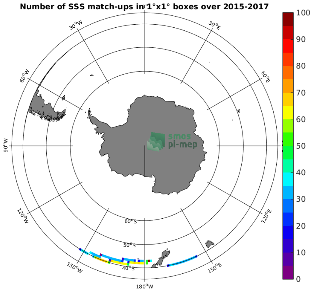
Figure 4: Number of SSS match-ups between TSG-LEGOS-DM SSS and the SMAP-L3-RSS-V3-8DAY-RUNNING-70KM SSS product for the Roaring Forties and Furious Fifties Pi-MEP region over 1°x1° boxes and for the full satellite product period.
